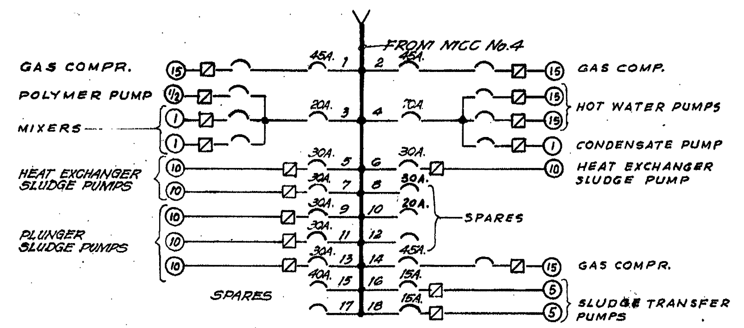
POWER PANEL-1 (PP-1)
