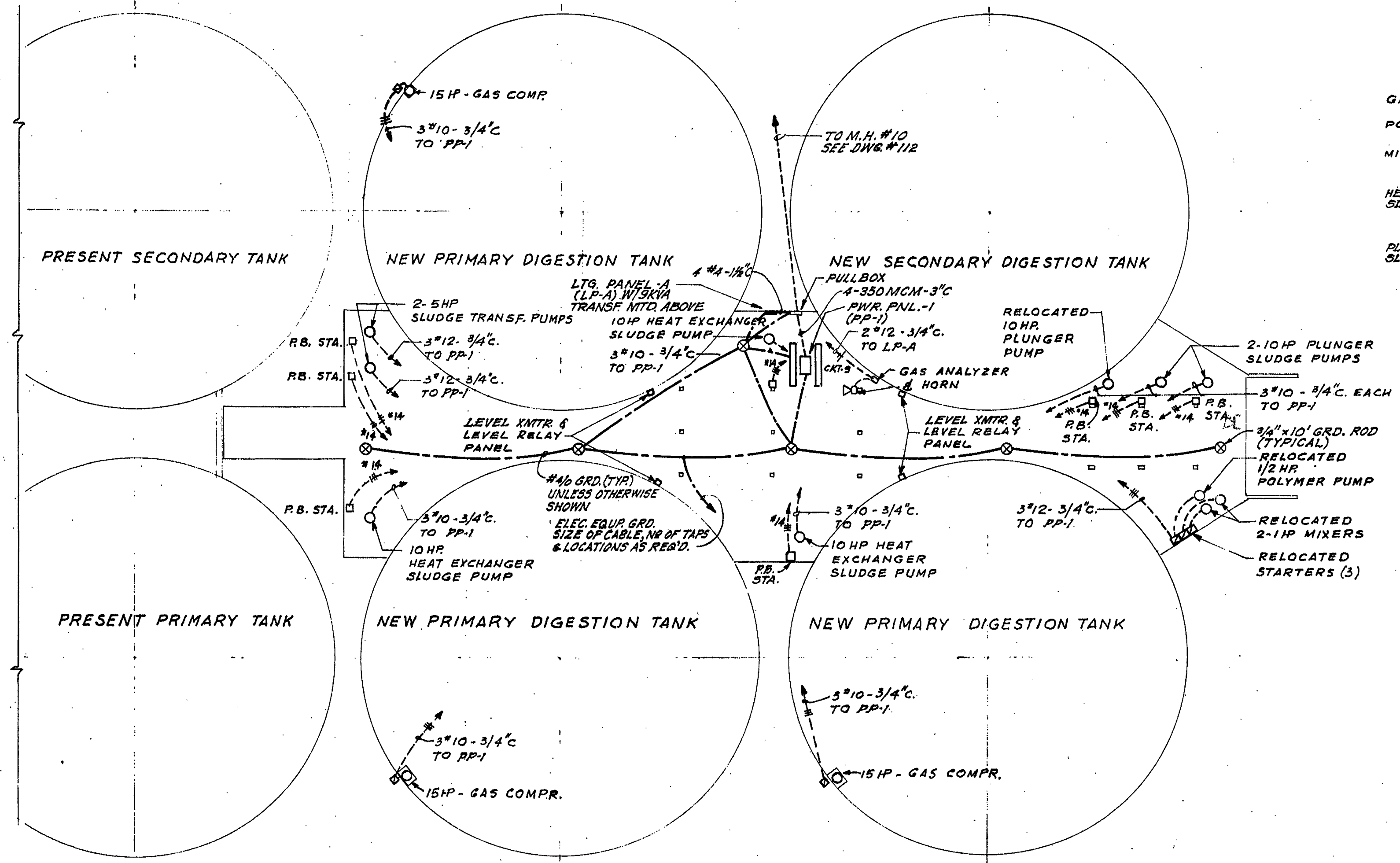
DIGESTER PLAN - FLOOR EL. 903.1 - POWER SCALE: 1" = 20'-0"
