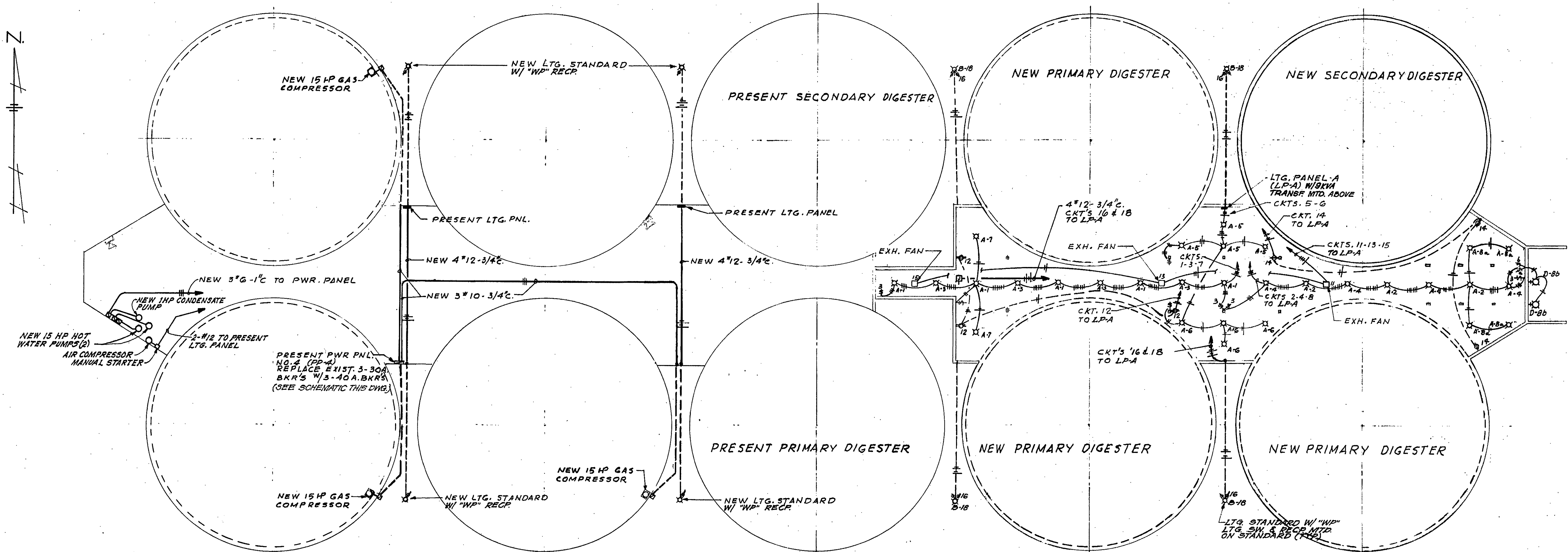
DIGESTER PLAN - FLOOR EL. 903.1 - LIGHTING SCALE: 1" = 20'-0"
