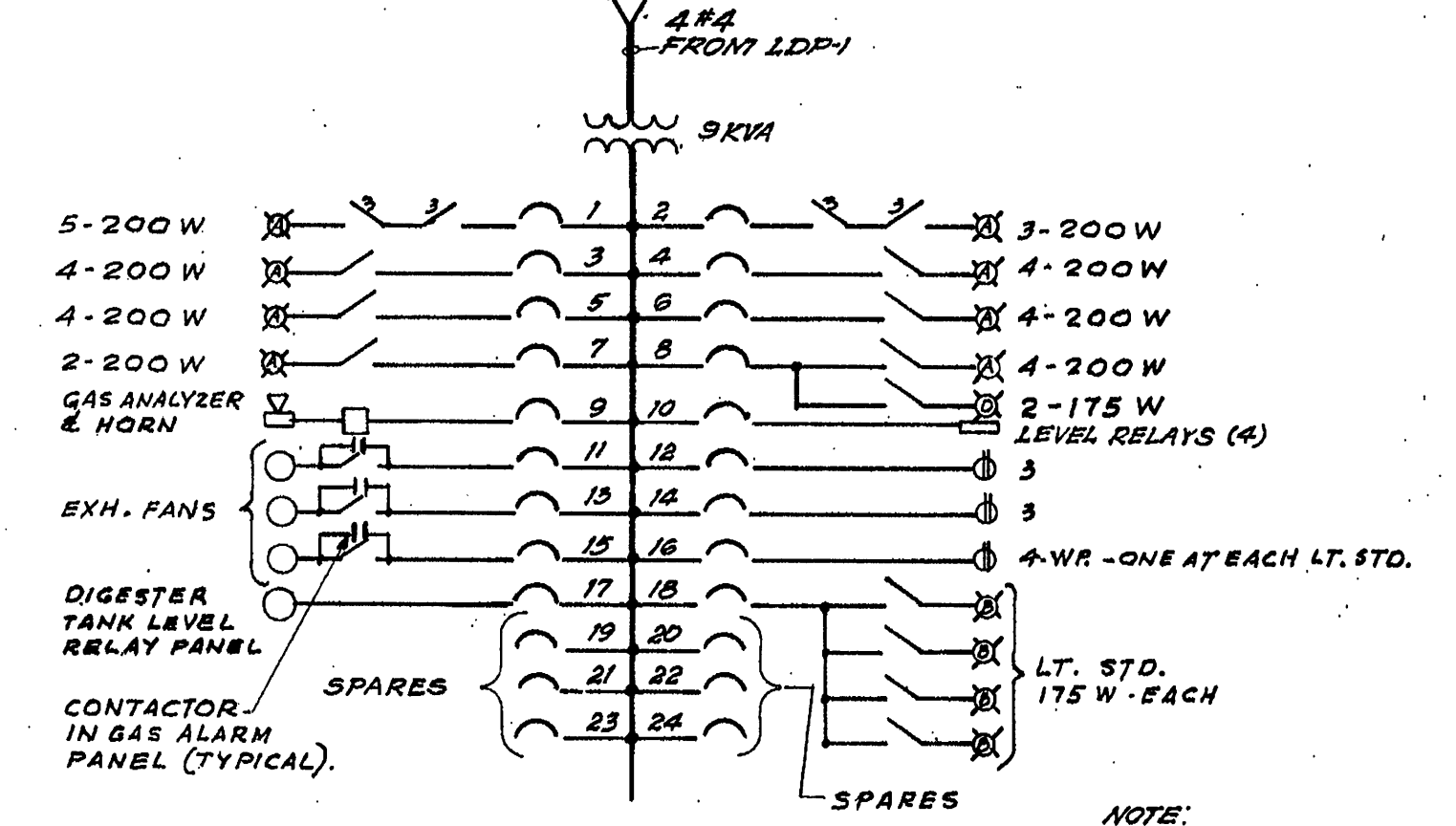
LIGHTING PANEL-A (LP-A)
