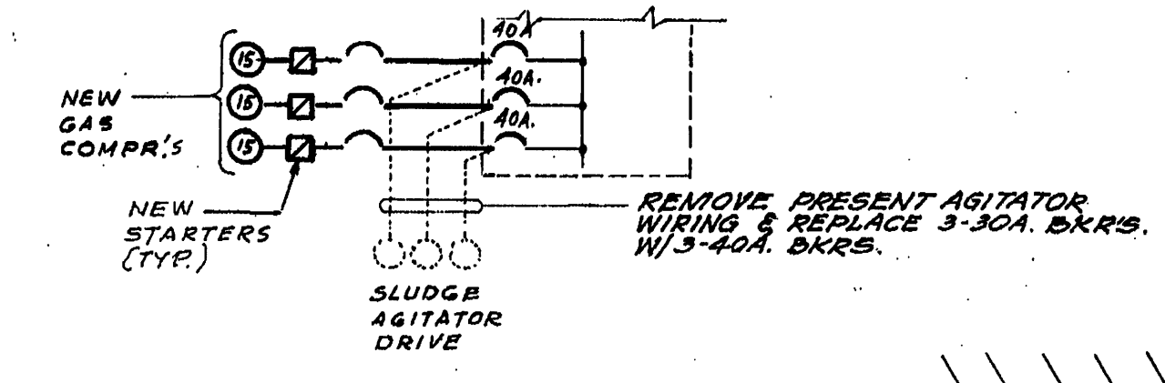
PRESENT POWER PNL No. 4
