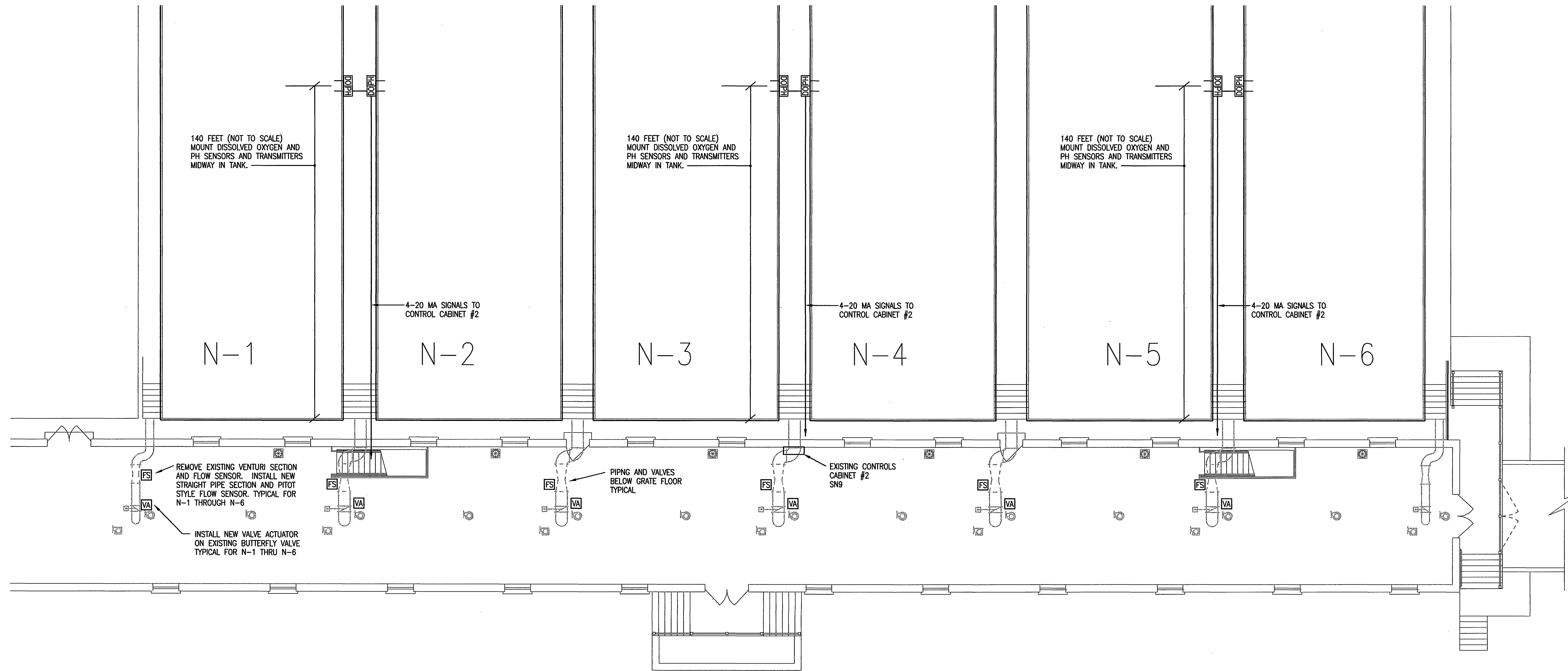
BLOWER BUILDING PARTIAL FLOOR PLAN - VALVE GALLERY 1/8"=1'-0"
