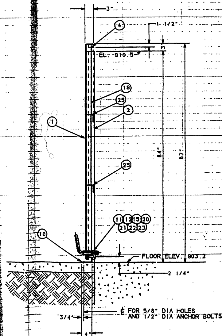
VERTICAL SECTION
