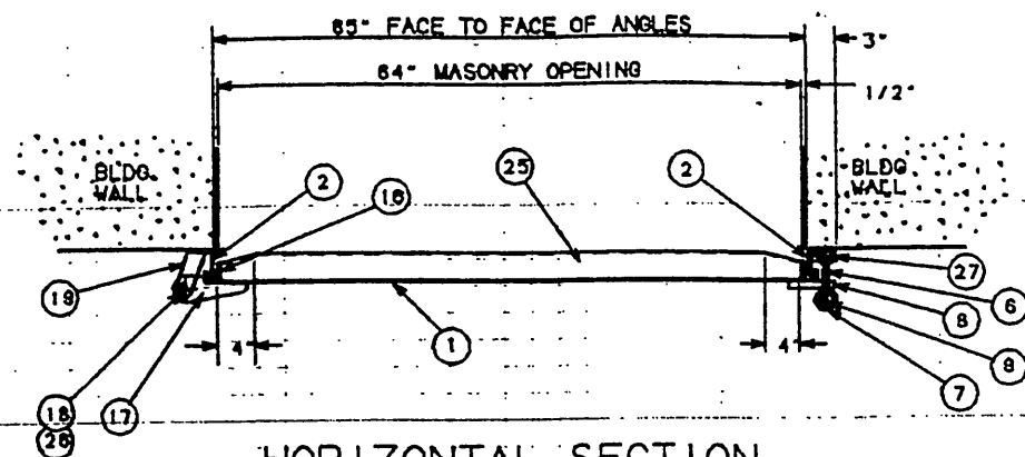
HORIZONTAL SECTION
