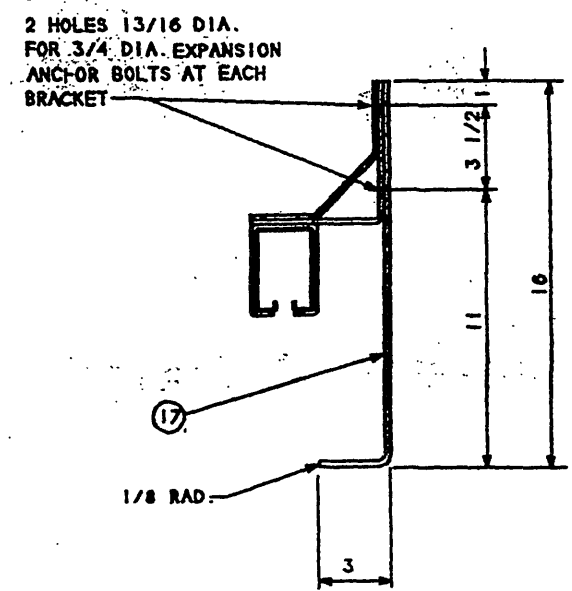
SECTION "H-H"
