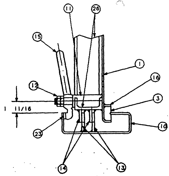
SECTION "D-D"
