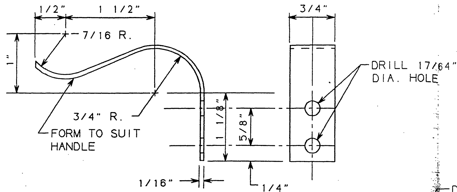
SPRING CLIP
