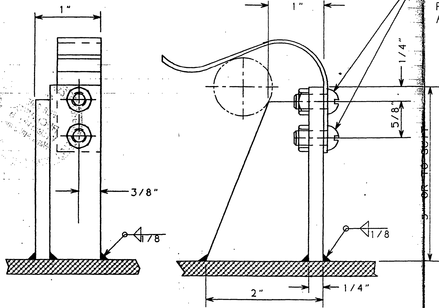
SPRING CLIP ASSEMBLY
