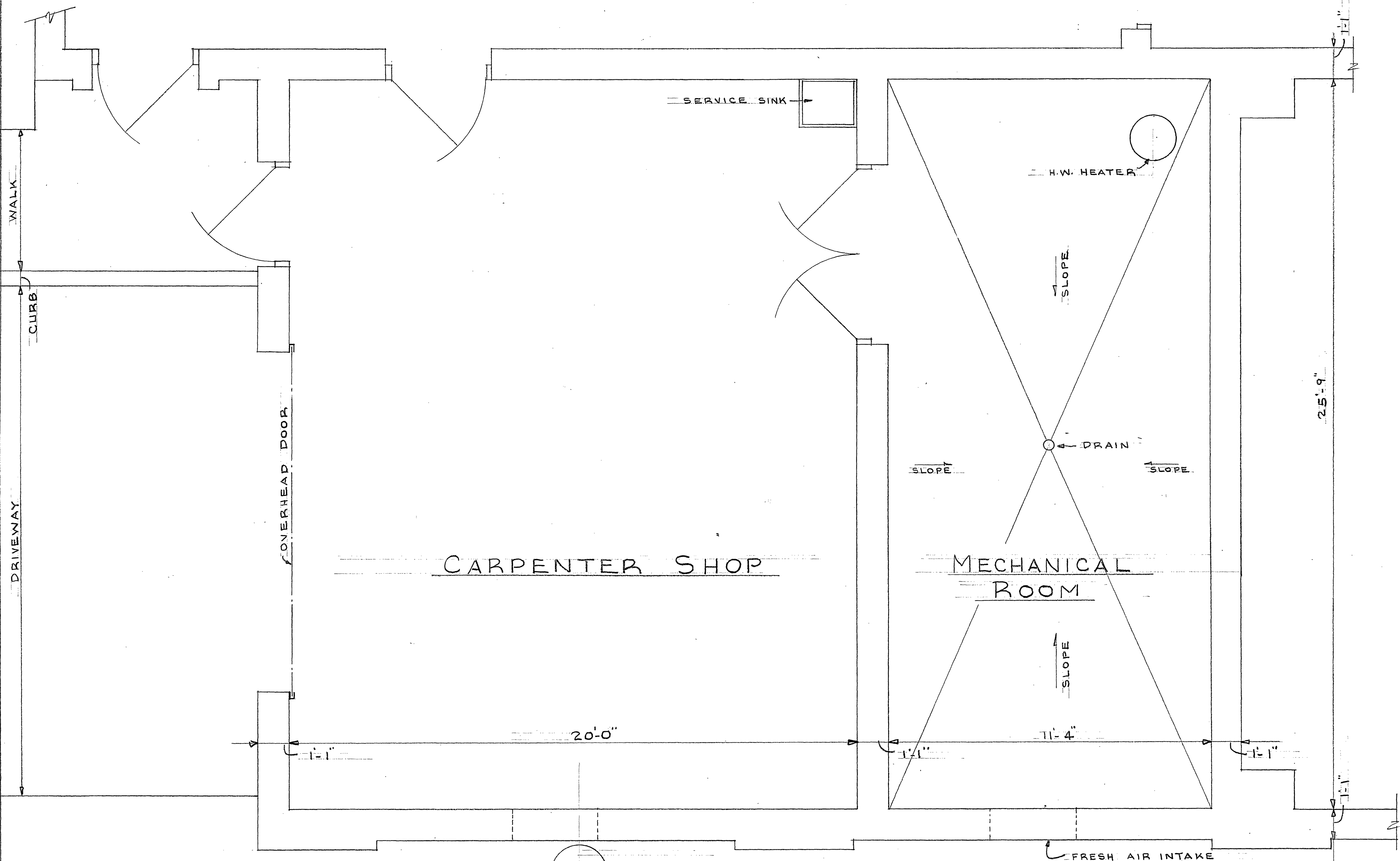
PARTIAL PLAN - SERVICE BUILDING SEWAGE TREATMENT PLANT SCALE : 1/2" = 1'-0"
