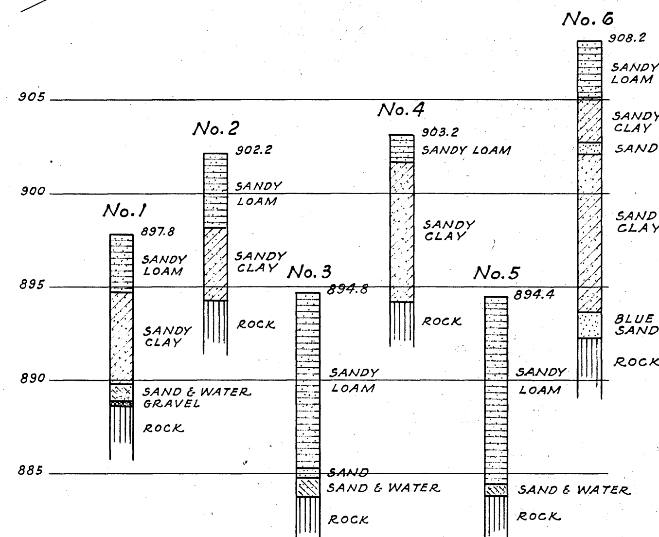
LOG OF TEST BORINGS
