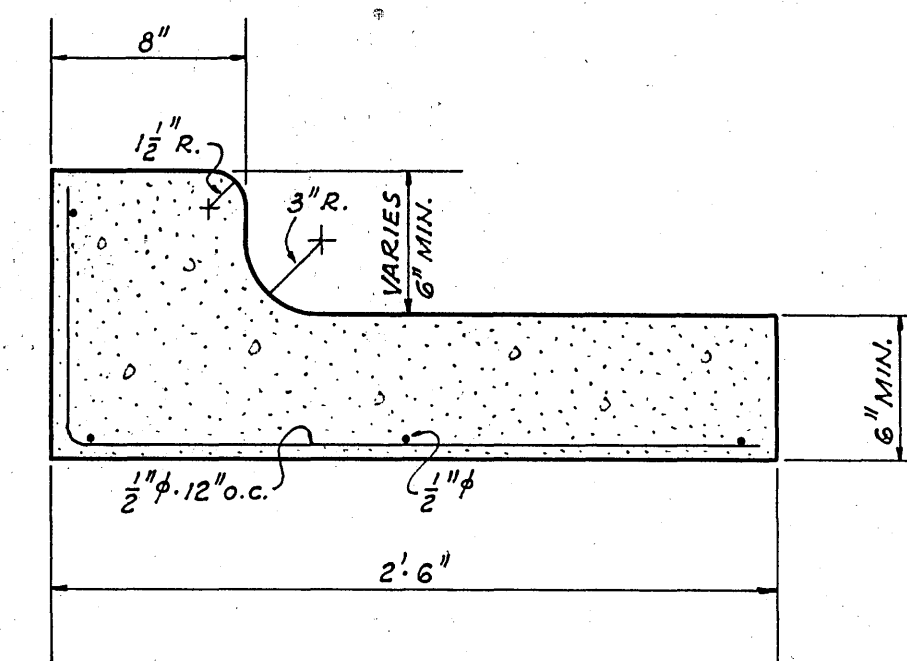
DETAIL OF CURB & GUTTER
