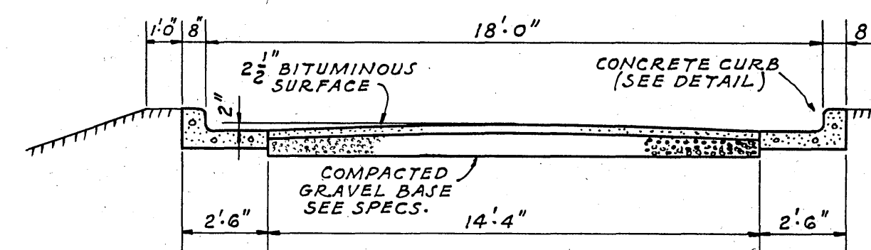
TYPICAL CROSS-SECTION OF ENTRANCE DRIVEWAY
