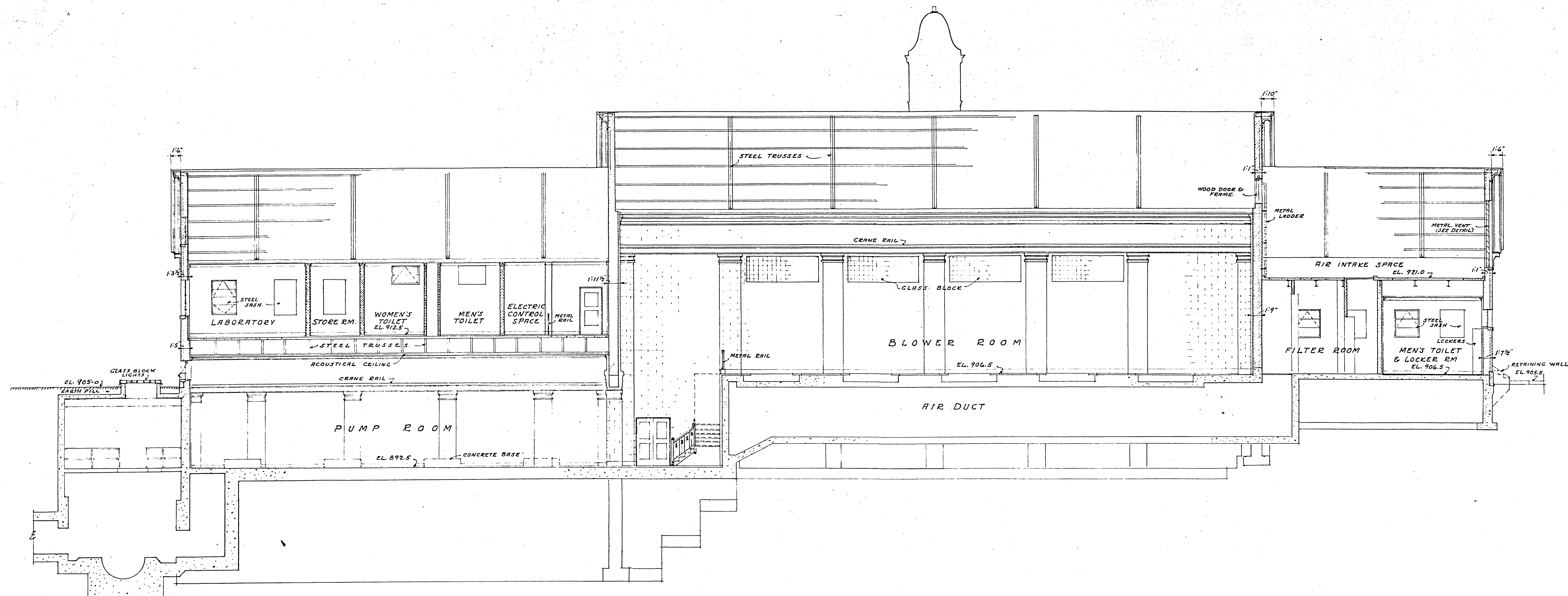
SECTION 1-1
