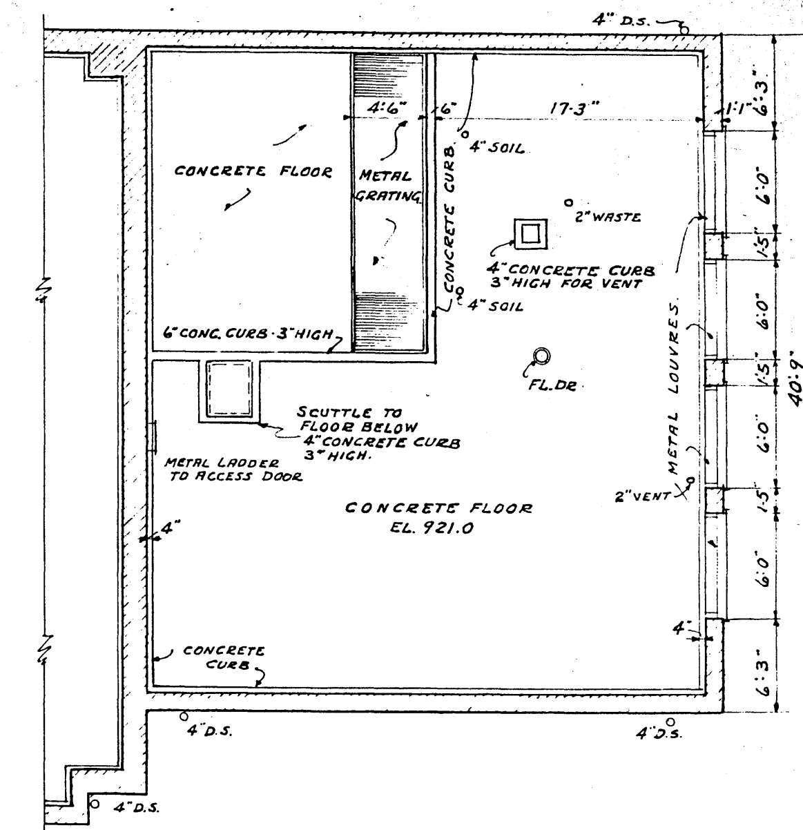
PLAN OF AIR INTAKE SPACE
