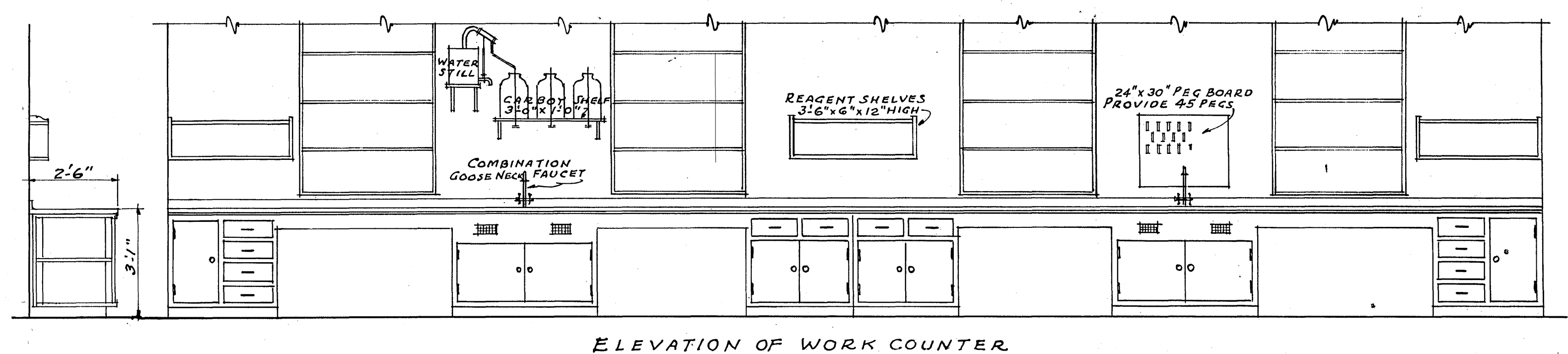
LABORATORY DETAILS SCALE 3/8" = 1'-0"
