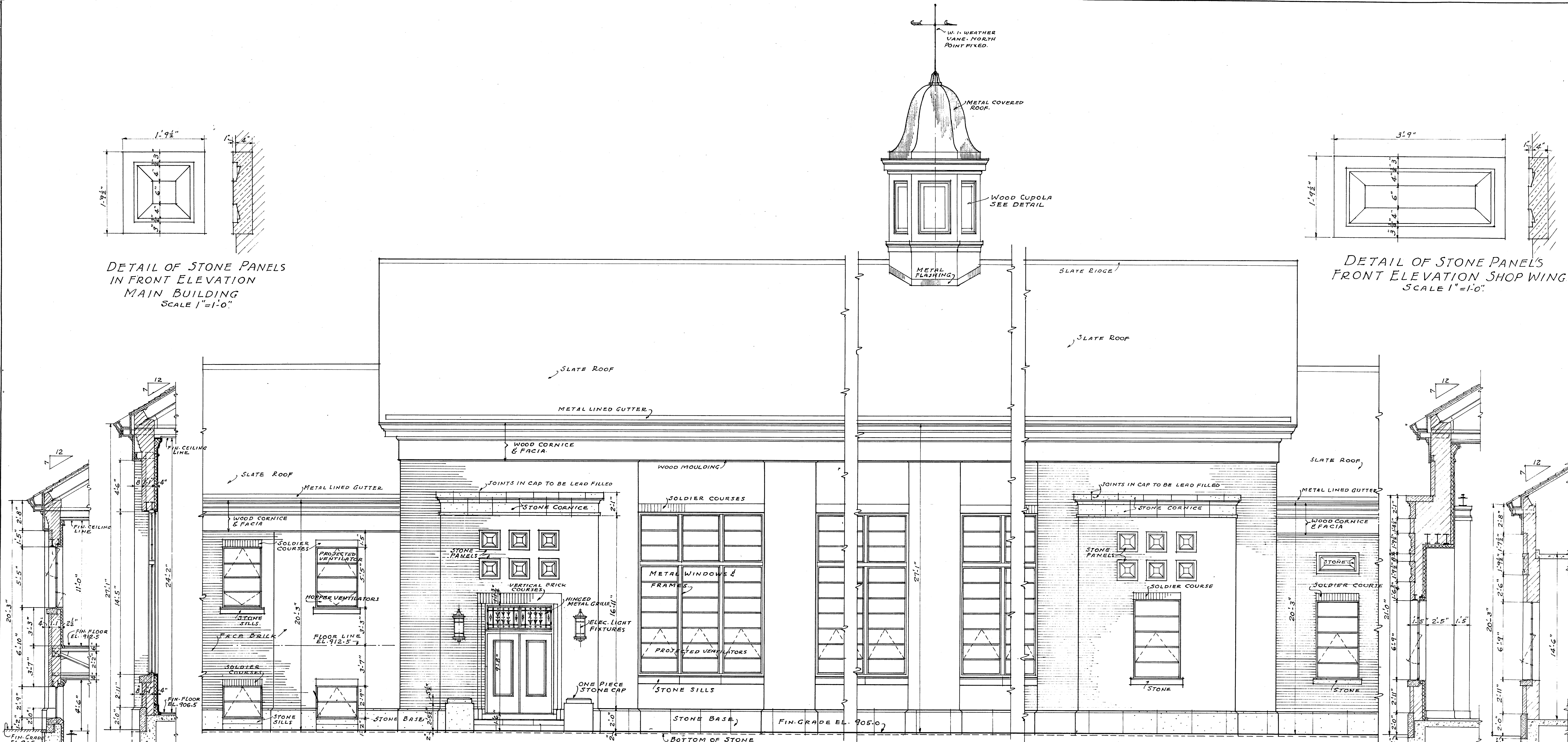
DETAIL OF FRONT ELEVATION BLOWER BUILDING. SCALE 1/4"=1'-0"
