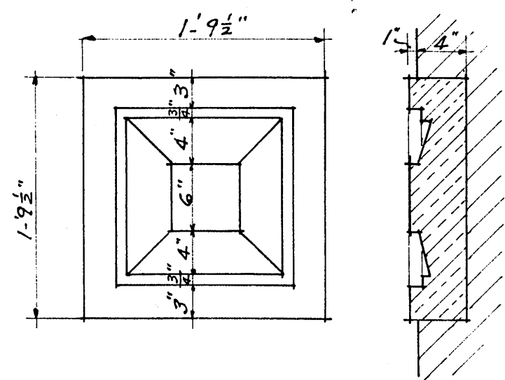
DETAIL OF STONE PANELS IN FRONT ELEVATION MAIN BUILDING SCALE 1"=1'-0"
