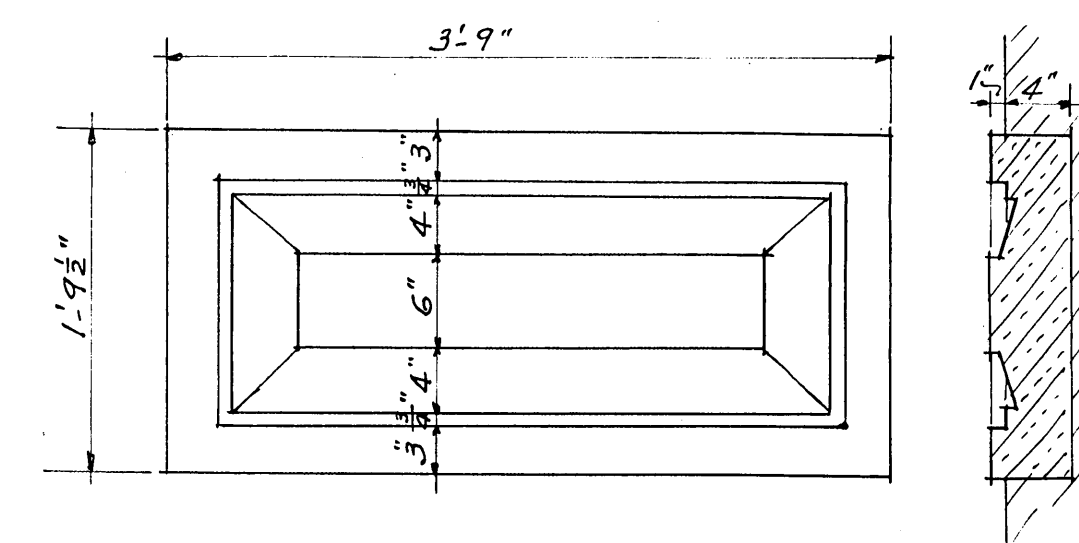
DETAIL OF STONE PANELS FRONT ELEVATION SHOP WING SCALE 1"=1'-0"
