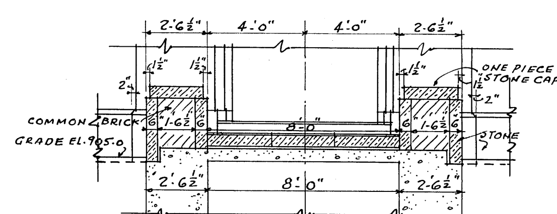
CROSS SECTION THRU BUTTRESSES AT MAIN ENTR. SCALE 1/4"=1'-0"
