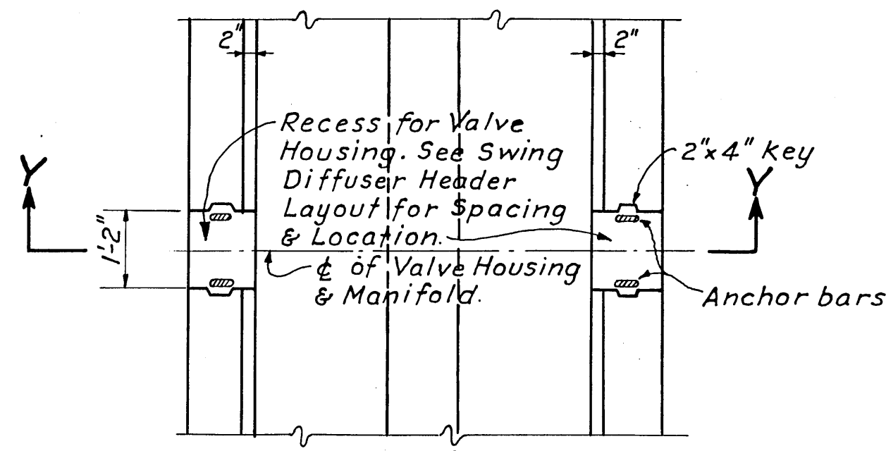
PLAN DETAIL OF COPING Scale: 1/2" = 1'-0"
