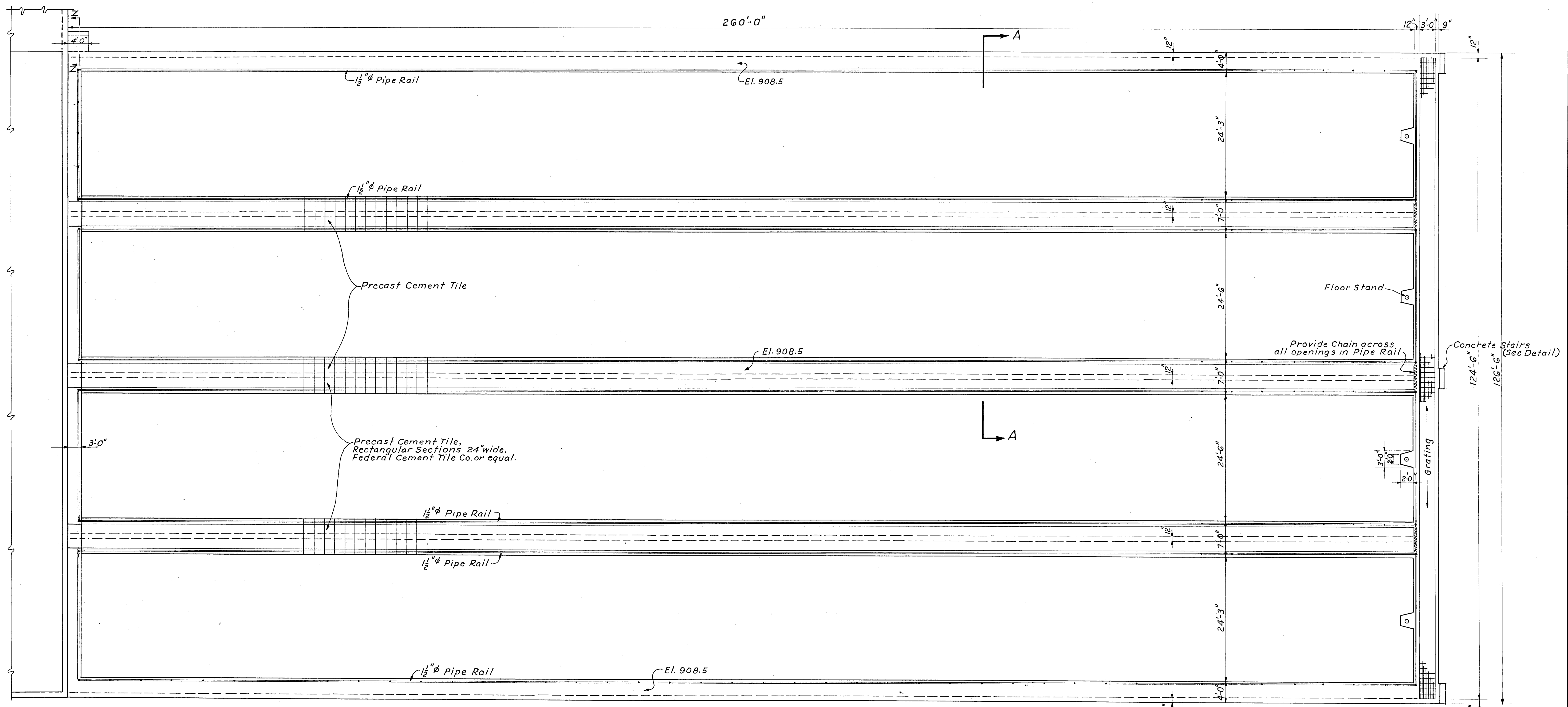
PLAN AT ELEV. 908.5 SCALE: 1" = 10'-0"
