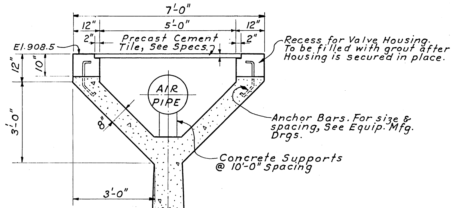
SECTION Y-Y
