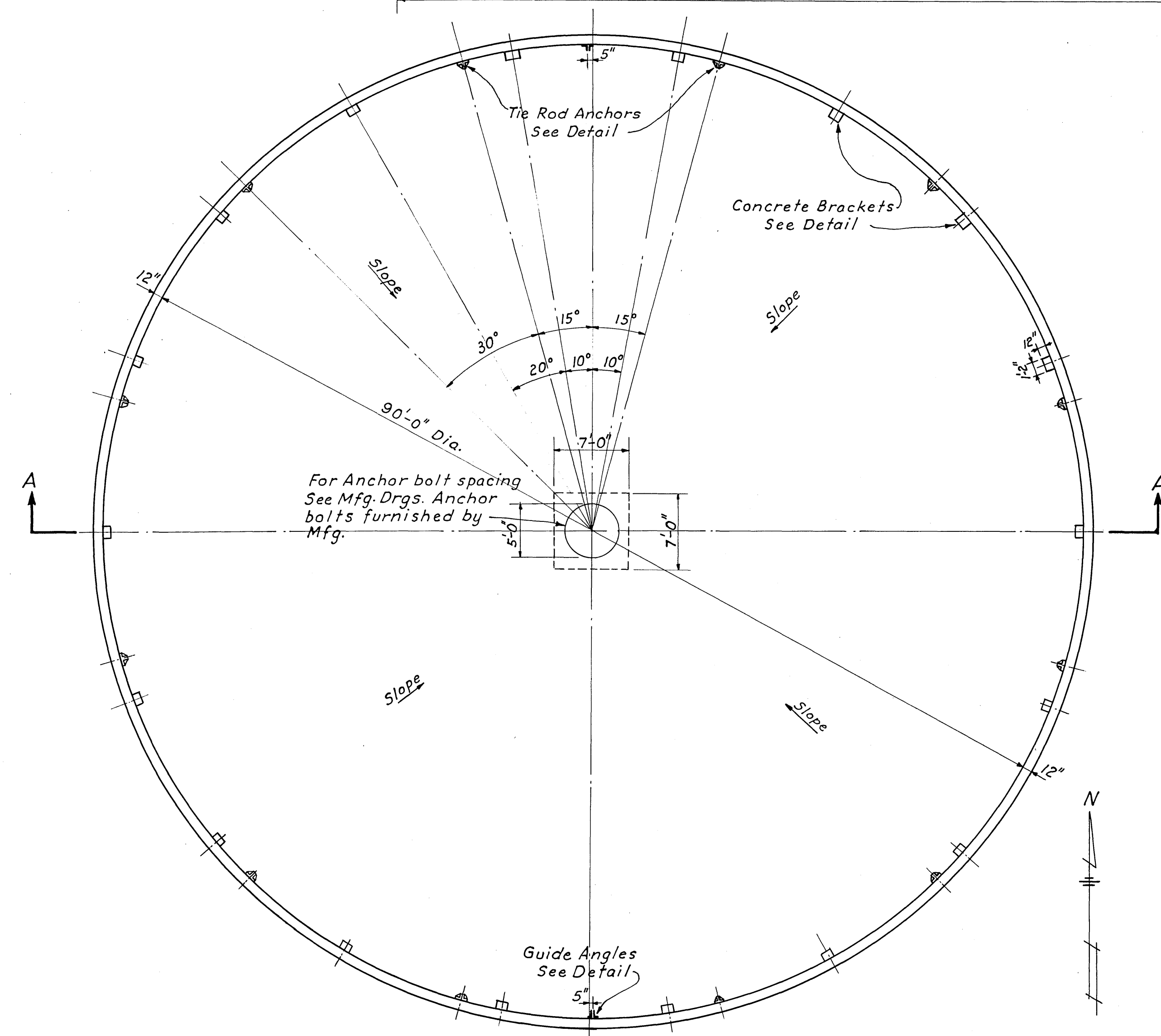
PLAN OF SECONDARY DIGESTION TANK ALTERNATE "A" Scale: \frac{1}{8}" = 1'-0"
