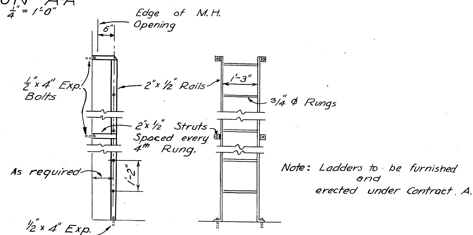
TYPICAL LADDER DETAIL Scale 1/2" = 1'-0"
