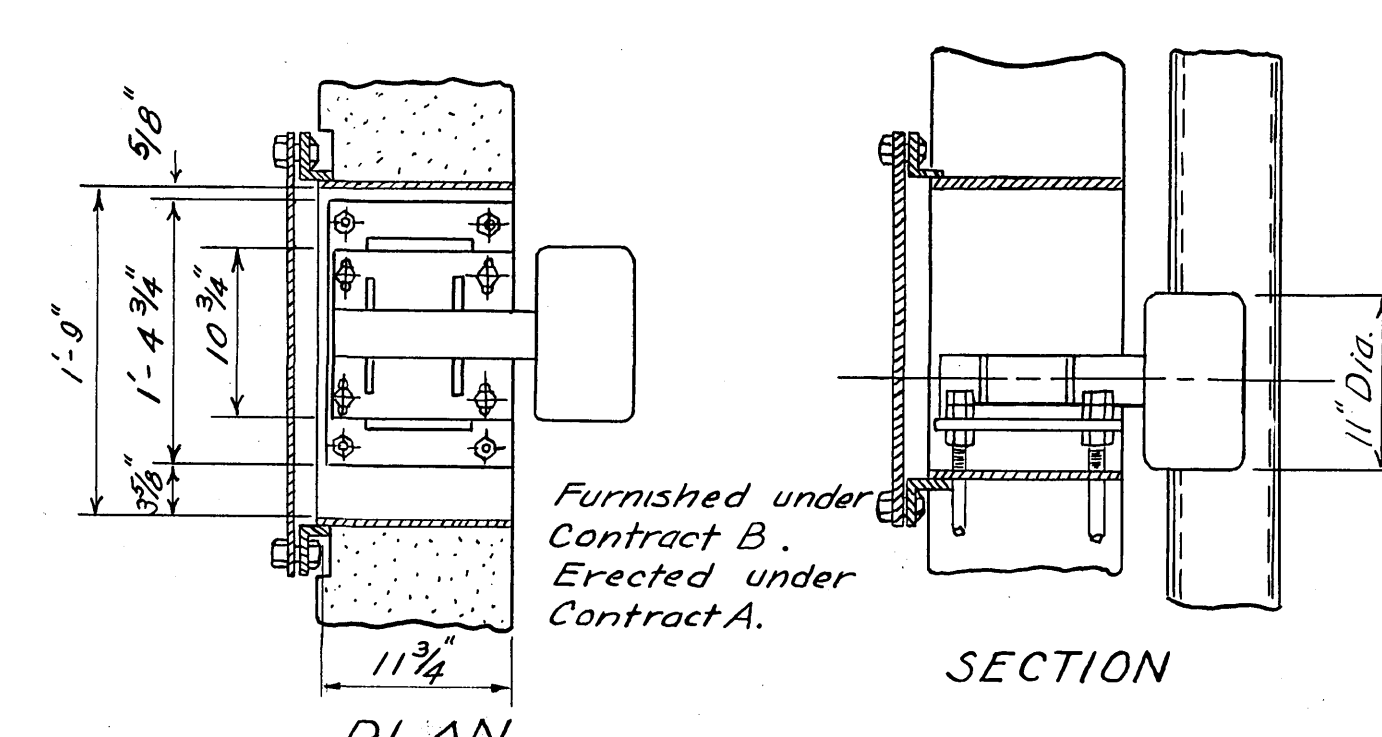
DETAIL OF ROLLER & BOX SECONDARY DIGESTION TANK ALTERNATE "B" Scale 1" = 1'-0"
