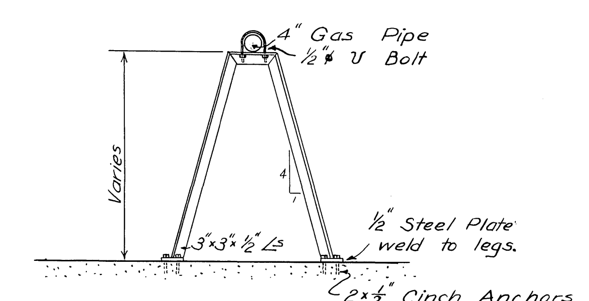
DETAIL OF GAS PIPE SUPPORT Scale 1/2" = 1'-0"
