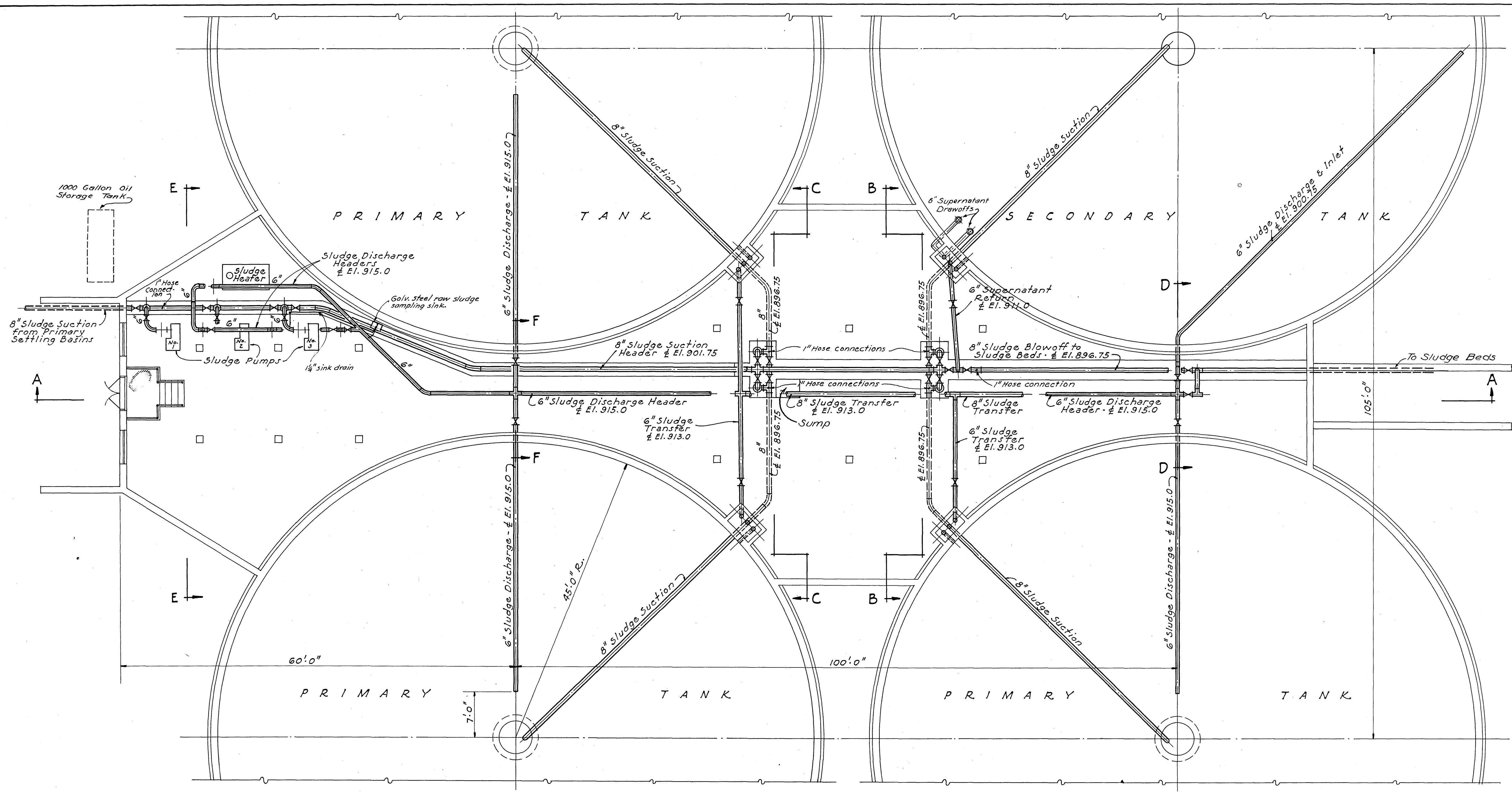
PLAN OF DIGESTION TANK SLUDGE PIPING SCALE: \frac{1}{8}" = 1'0"
