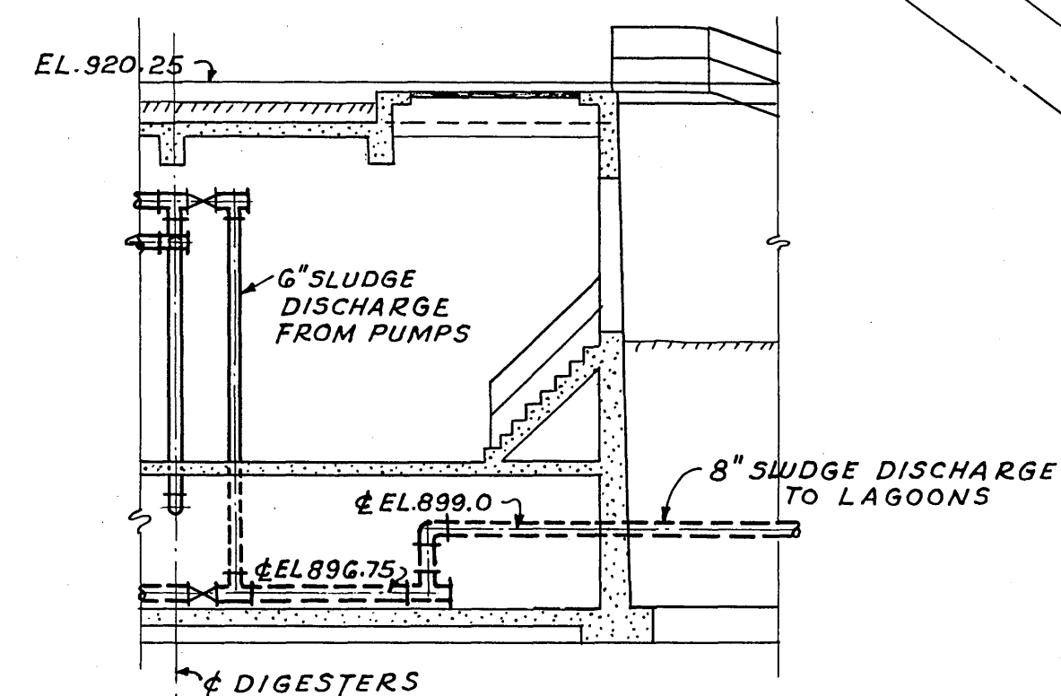
DETAIL OF DIGESTER CONTROL HOUSE SCALE: 1/8" = 1'-0"
