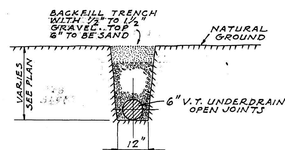
TYPICAL CROSS-SECTION OF UNDERDRAIN TRENCH SCALE: 1/2" = 1'-0"
