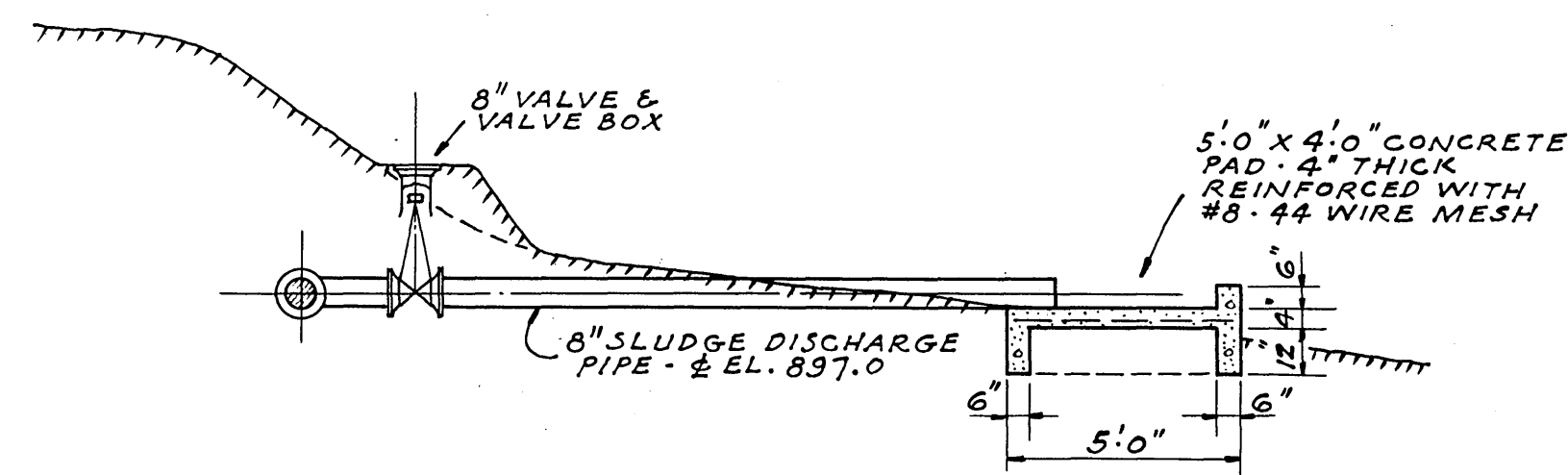
TYPICAL DETAIL OF DISCHARGE TO LAGOON SCALE: 1/4" = 1'-0"
