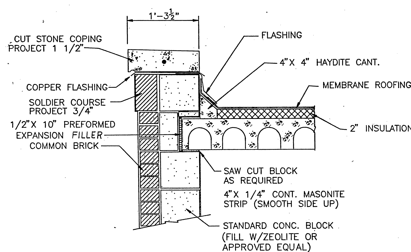
TYPICAL WALL SECTION 6 7 SCALE: 3/4" = 1'
