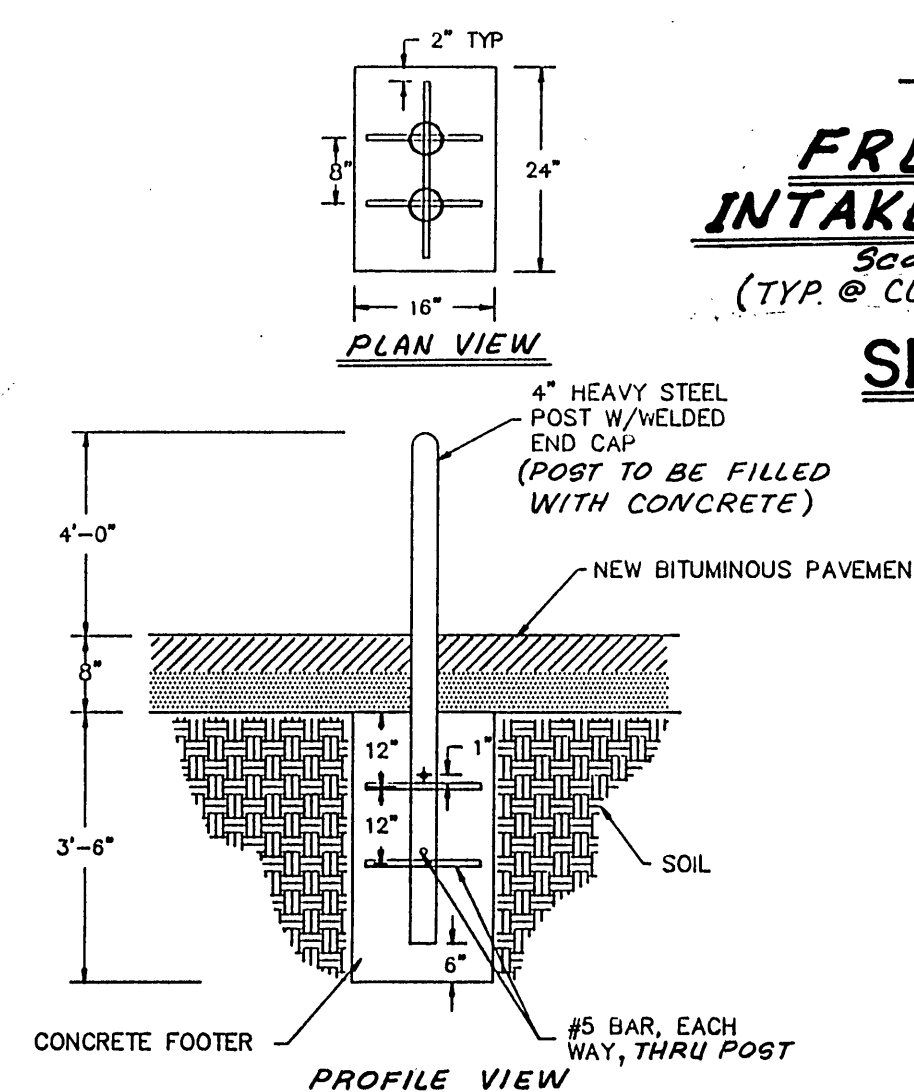
GUARD POST DETAIL NOT TO SCALE
