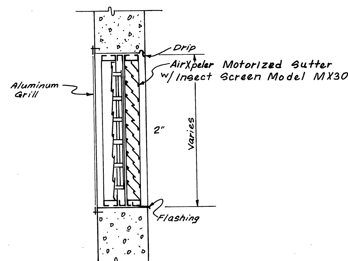
FRESH AIR INTAKE LOUVER Scale: 3/4" = 1'-0" (TYP. @ CL 2 , 80 2 , & CONTROL RM.) SECTION 9 7
