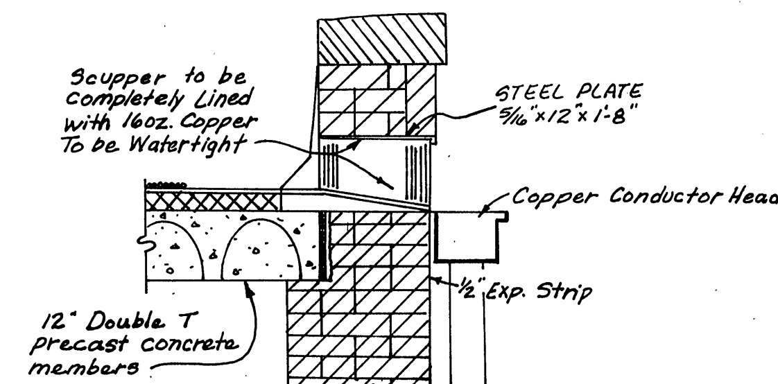
SCUPPER DETAIL 7 7 SCALE: 3/4" = 1'-0"
