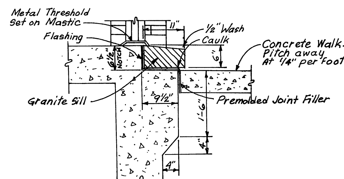
ENTRANCE DOOR DETAILS 8 7 SCALE: 3/4" = 1'-0"
