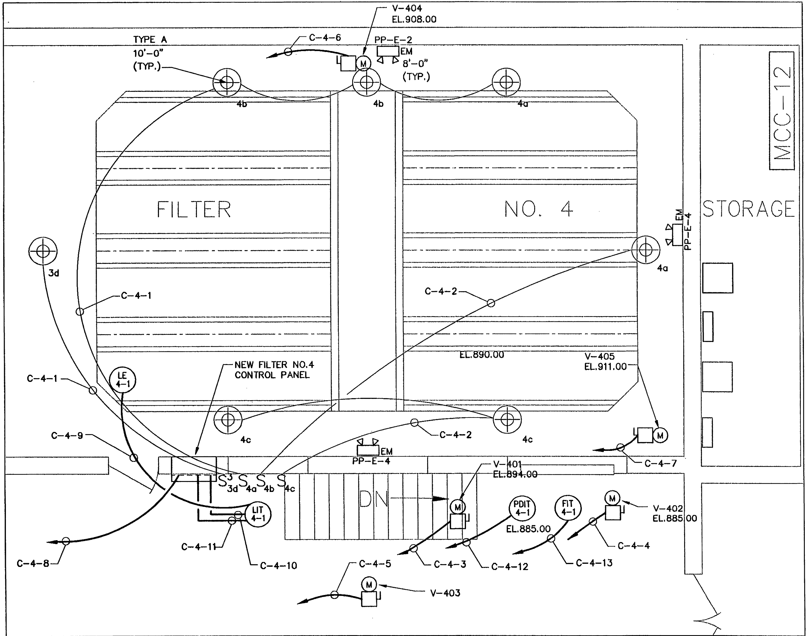
PARTIAL PLAN (TYPICAL FOR OTHER FILTERS) SCALE: 1/4" = 1'-0" SEE NOTE 2
