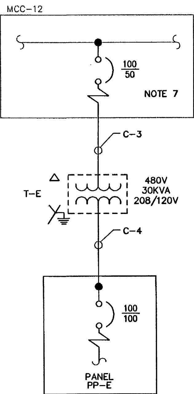
SINGLE LINE PP-E PANEL SCHEDULE ON SHEET E-1
