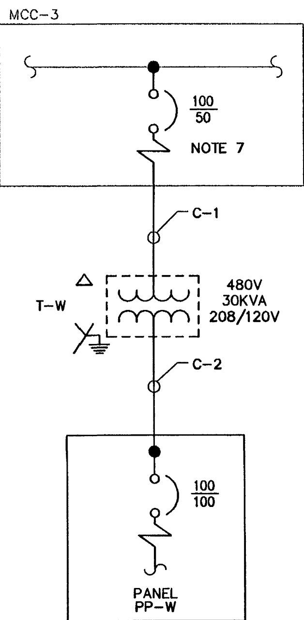
SINGLE LINE PP-W PANEL SCHEDULE ON SHEET E-1
