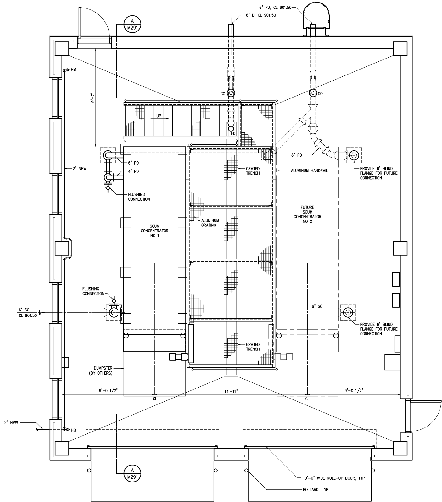
BOTTOM PLAN 3/8"=1'-0"
