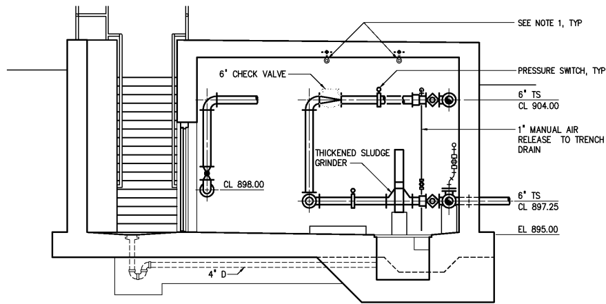
SECTION A 1/4"=1'-0" M720
