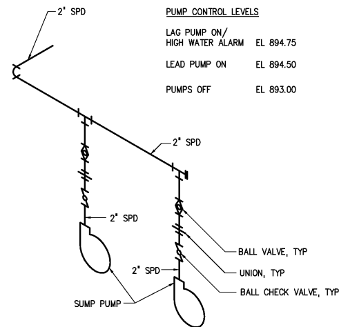
SUMP PUMP SCHEMATIC
