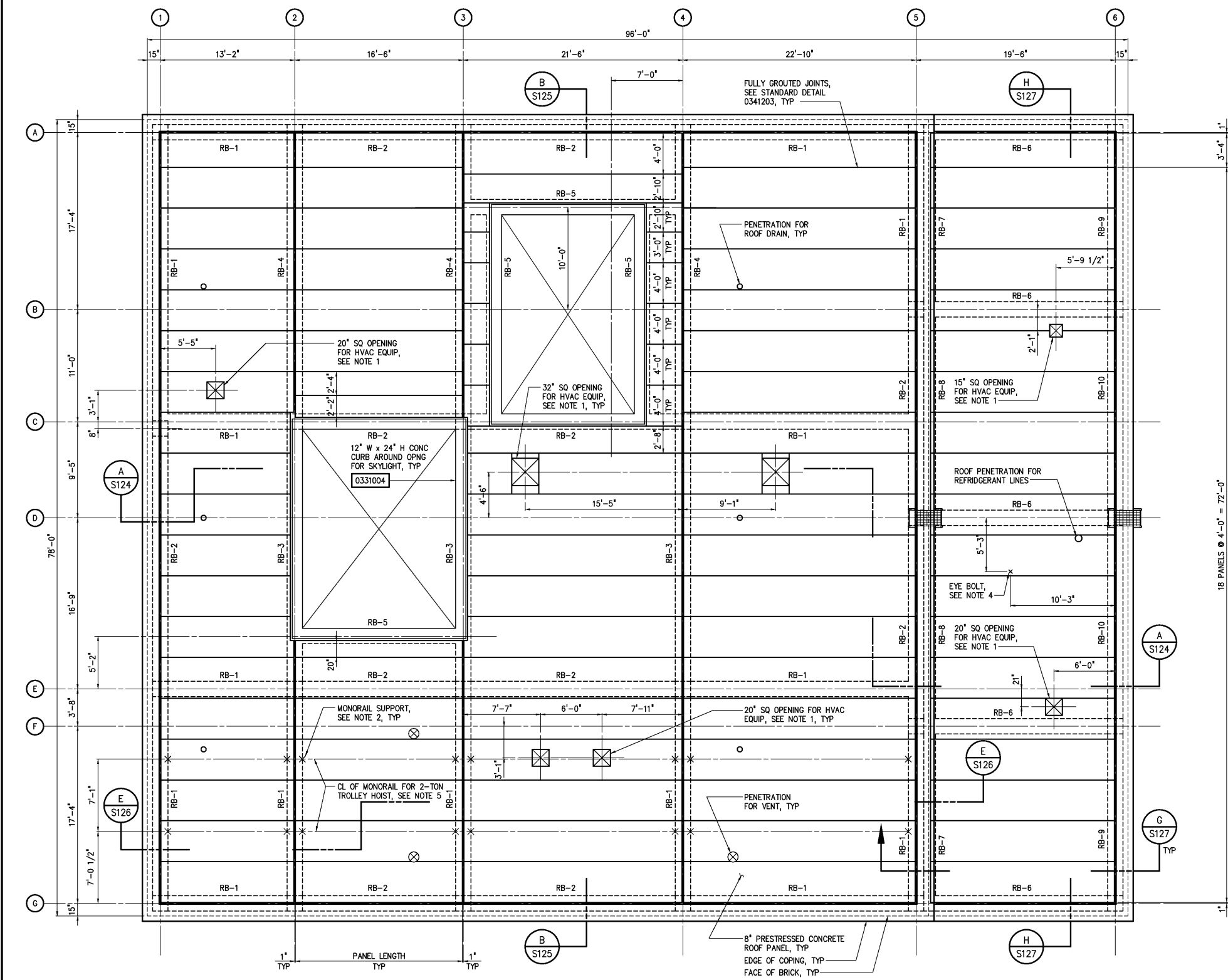
ROOF PLAN 3/16"=1'-0"
