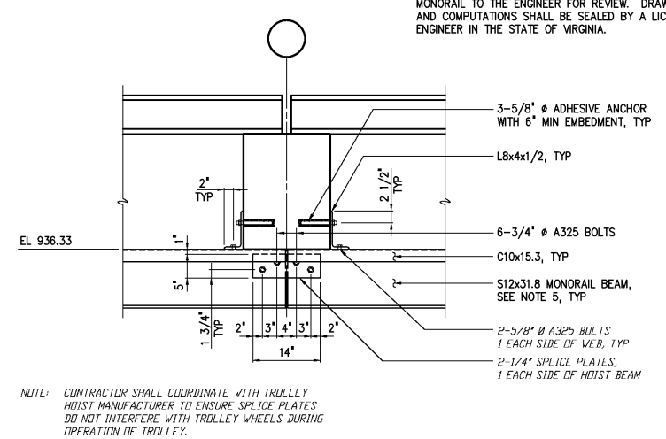
DETAIL 10 3/4"=1'-0" S126
