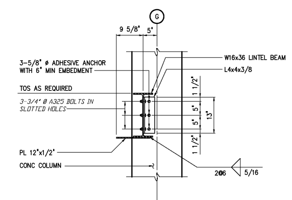
DETAIL 12 3/4"=1'-0" S125
