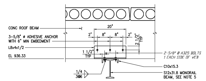
DETAIL 11 3/4"=1'-0" S125
