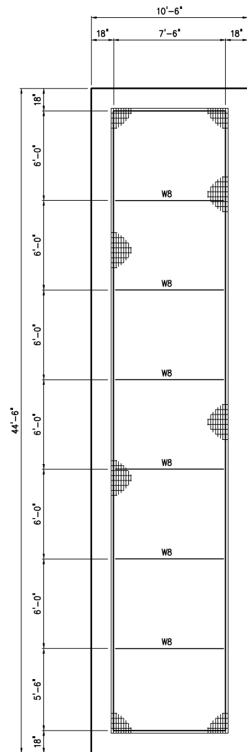
FRAMING PLAN – ELEVATION 922.00 1/4"=1'-0"
