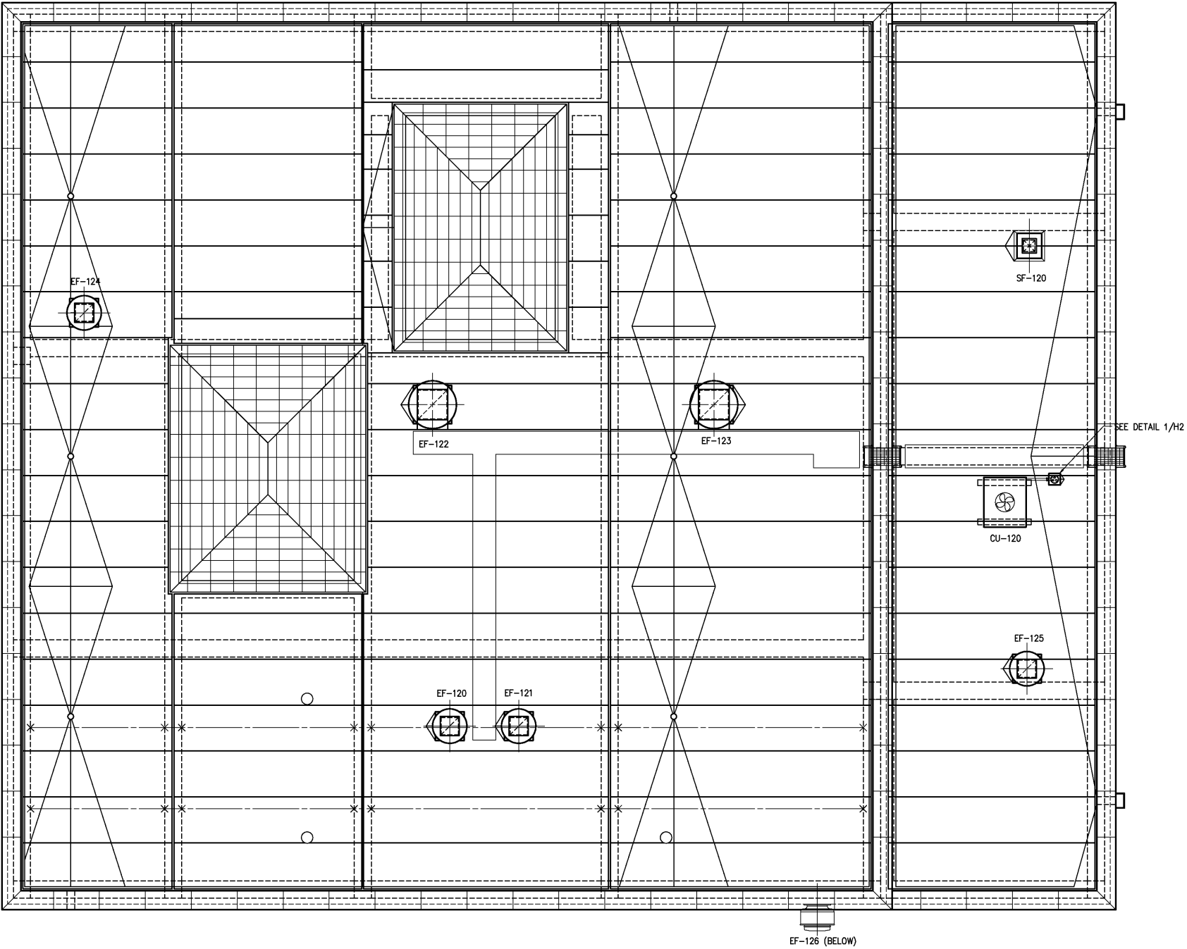
ROOF PLAN 3/16"=1'-0"
