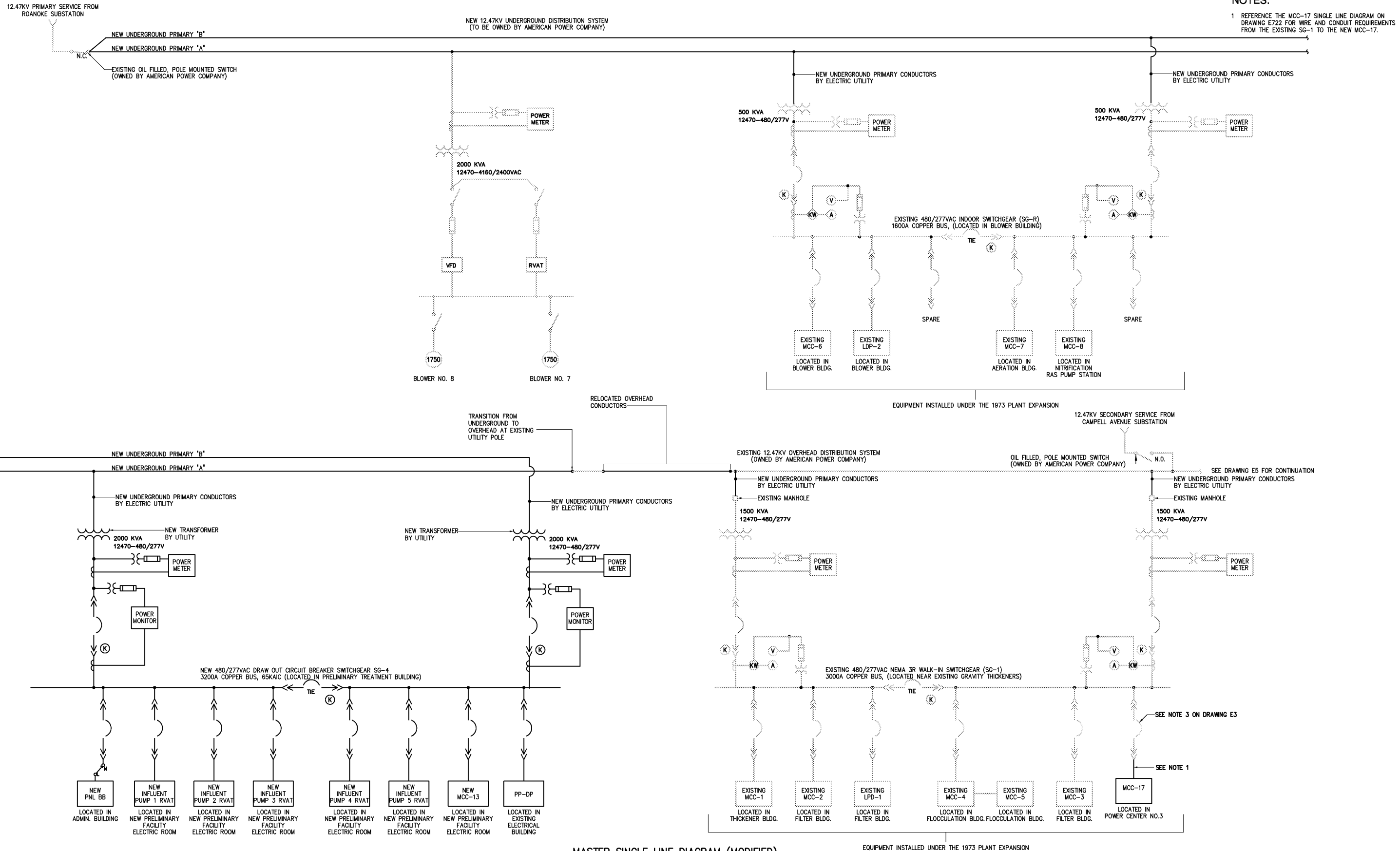
MASTER SINGLE LINE DIAGRAM (MODIFIED)
