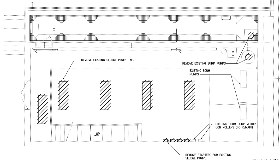
BOTTOM PLAN-DEMOLITION
