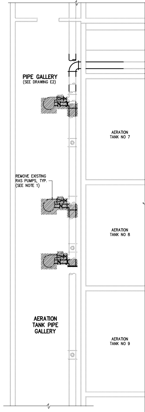
PARTIAL PLAN DEMOLITION
