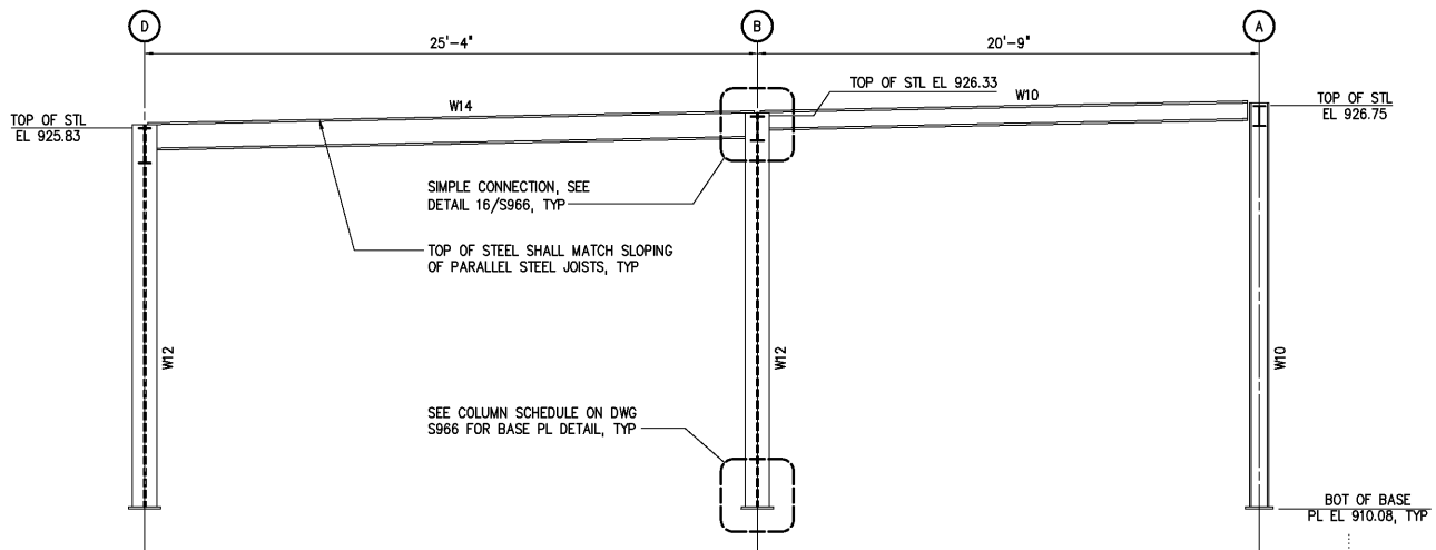
STEEL ELEVATION AT COL LINES 4, 5, 6 & 7 1/4"=1'-0"
