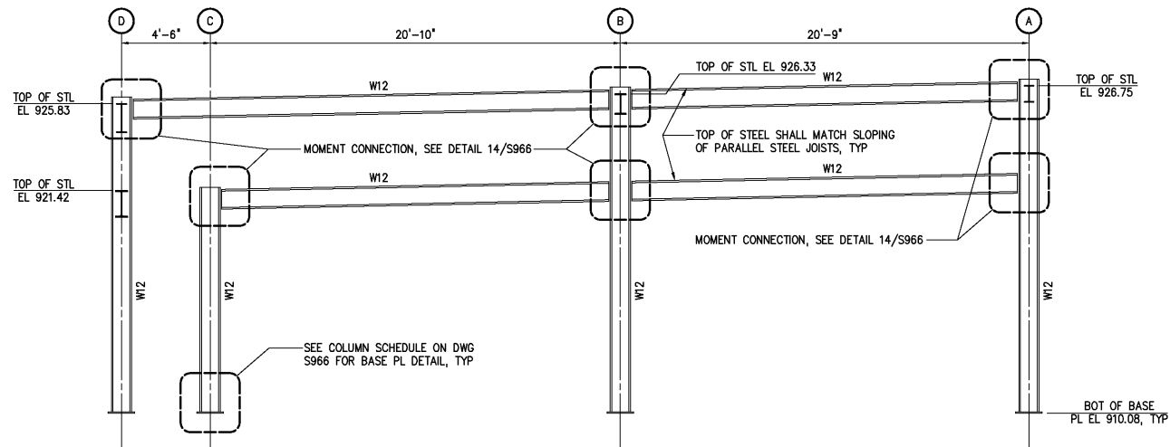
STEEL ELEVATION AT COL LINE 3 1/4"=1'-0"
