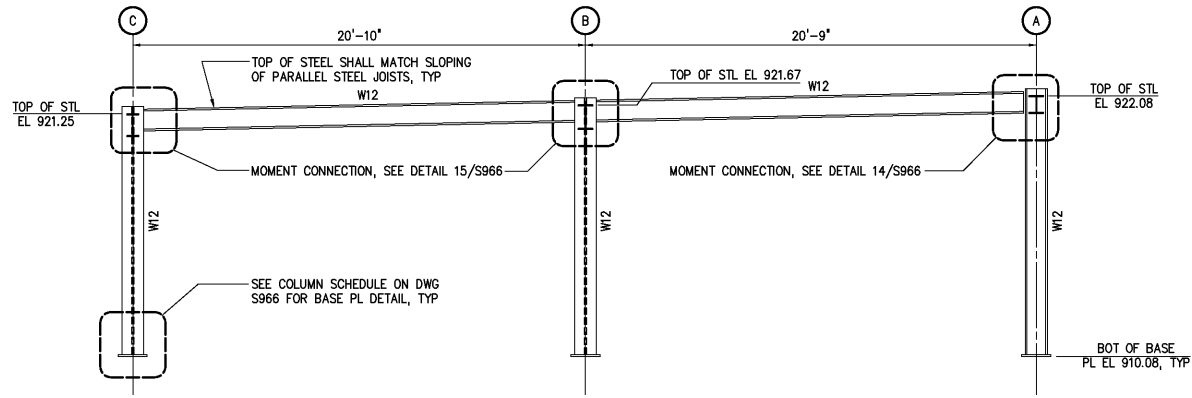
STEEL ELEVATION AT COL LINE 1 1/4"=1'-0"
