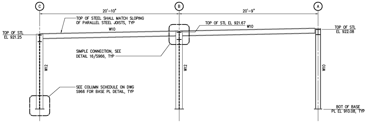
STEEL ELEVATION AT COL LINE 2 1/4"=1'-0"
