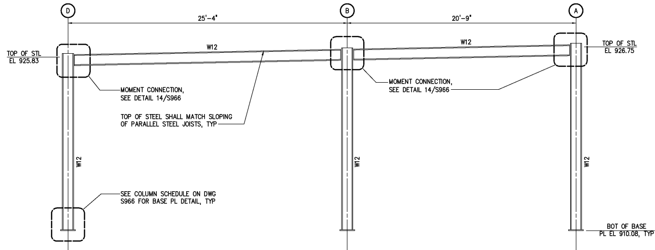
STEEL ELEVATION AT COL LINE 8 1/4"=1'-0"
