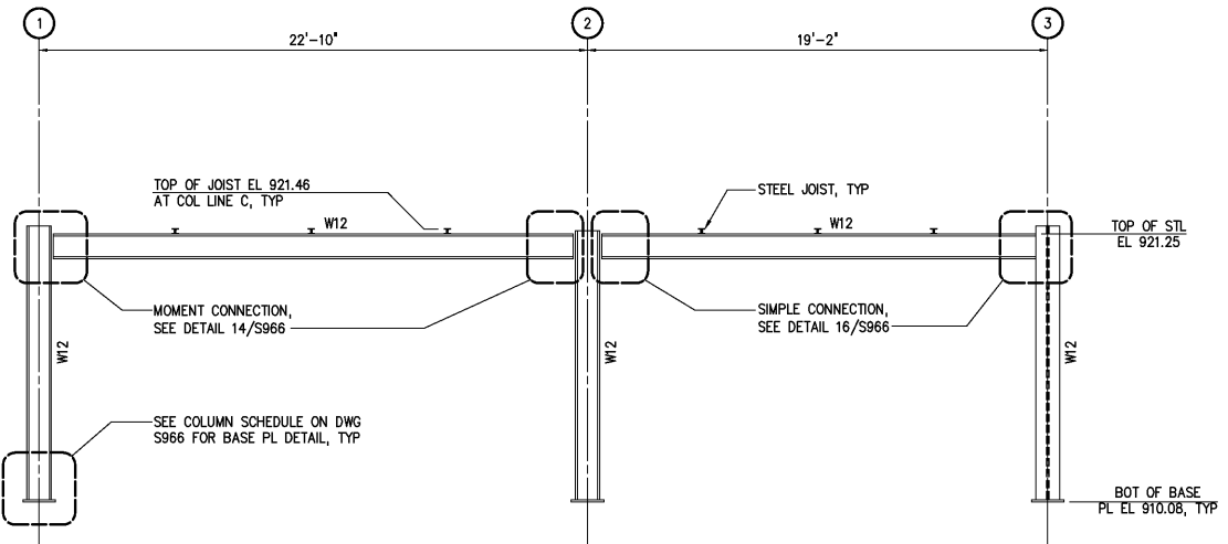
STEEL ELEVATION AT COL LINE C 1/4"=1'-0"
