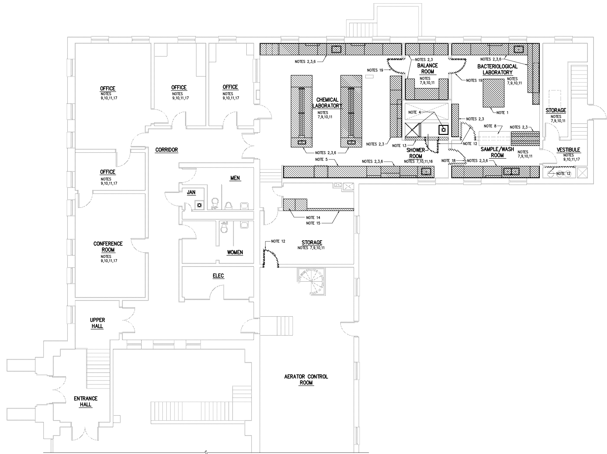
DEMOLITION PLAN 3/16"=1'-0"
