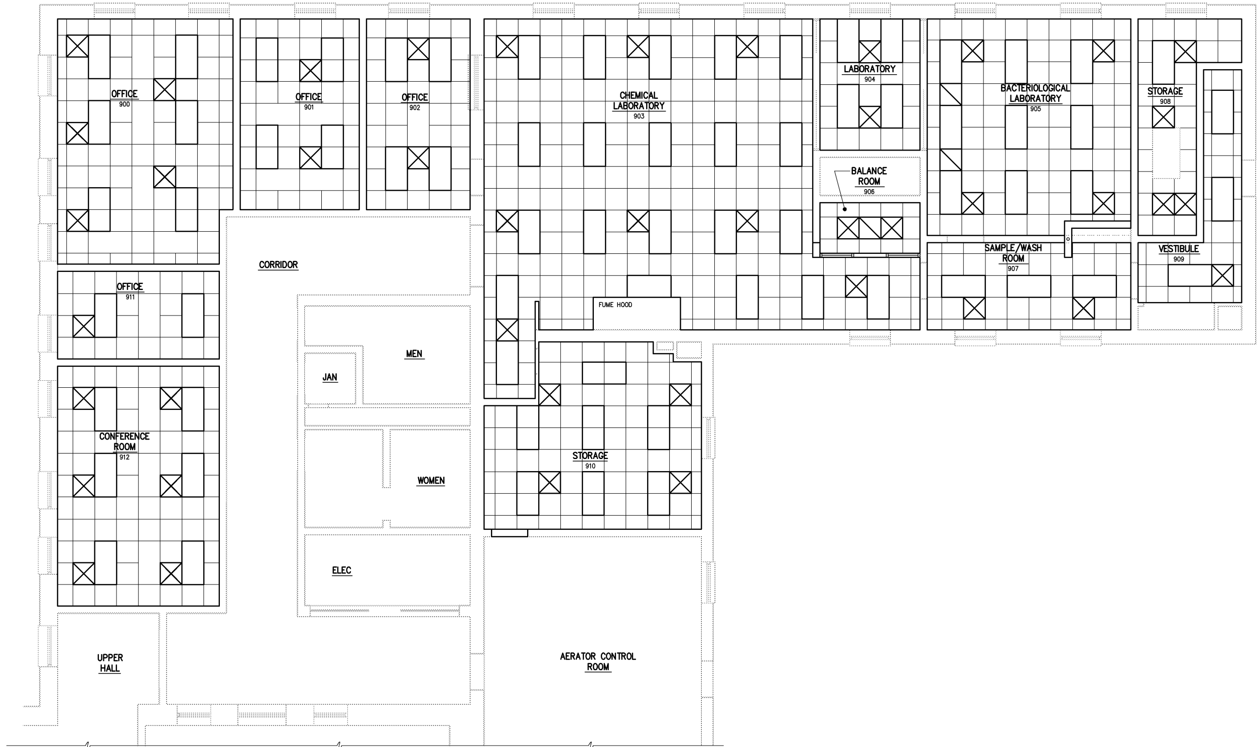
REFLECTED CEILING PLAN 1/4"=1'-0"
