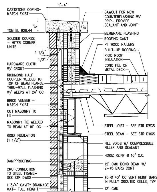
TYPICAL PARAPET DETAIL 153 1"=1'-0" A965
