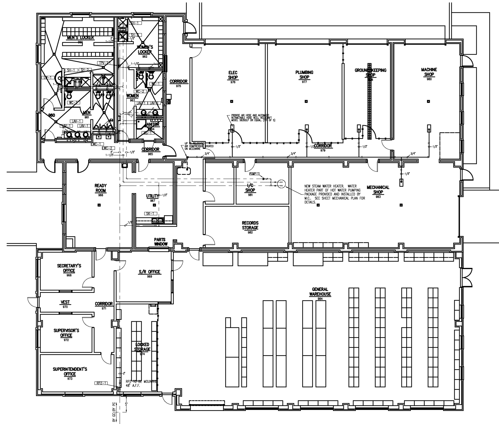
DOMESTIC WATER PLUMBING PLAN 1/8"=1'-0"
