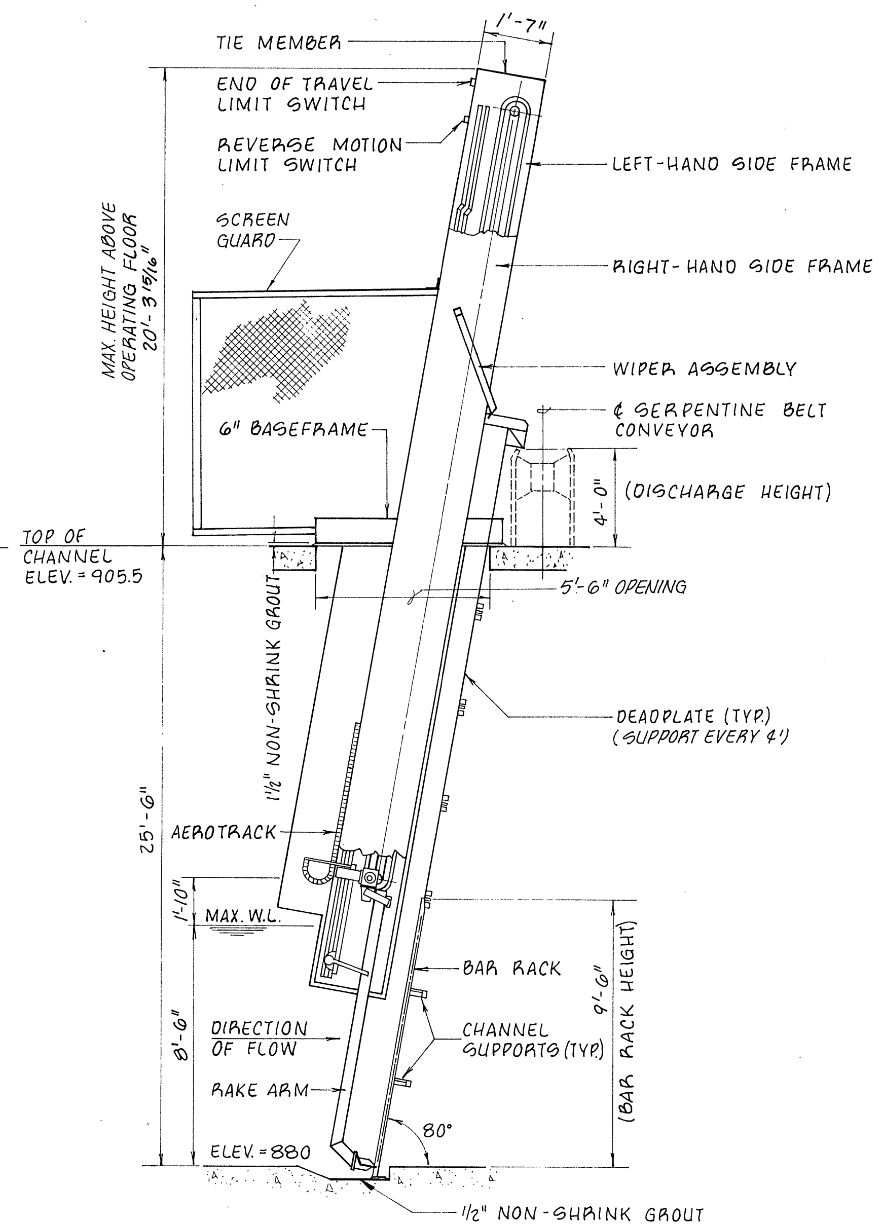
RIGHT SIDE ELEVATION
