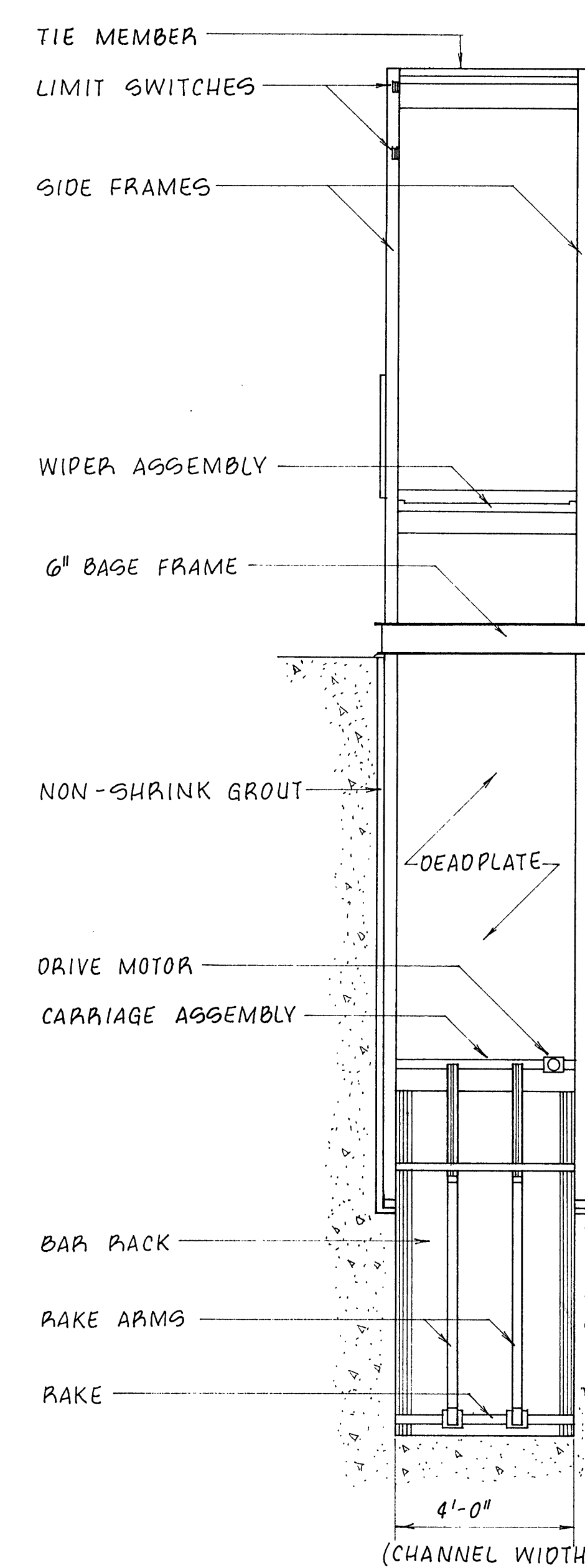
FRONT ELEVATION
