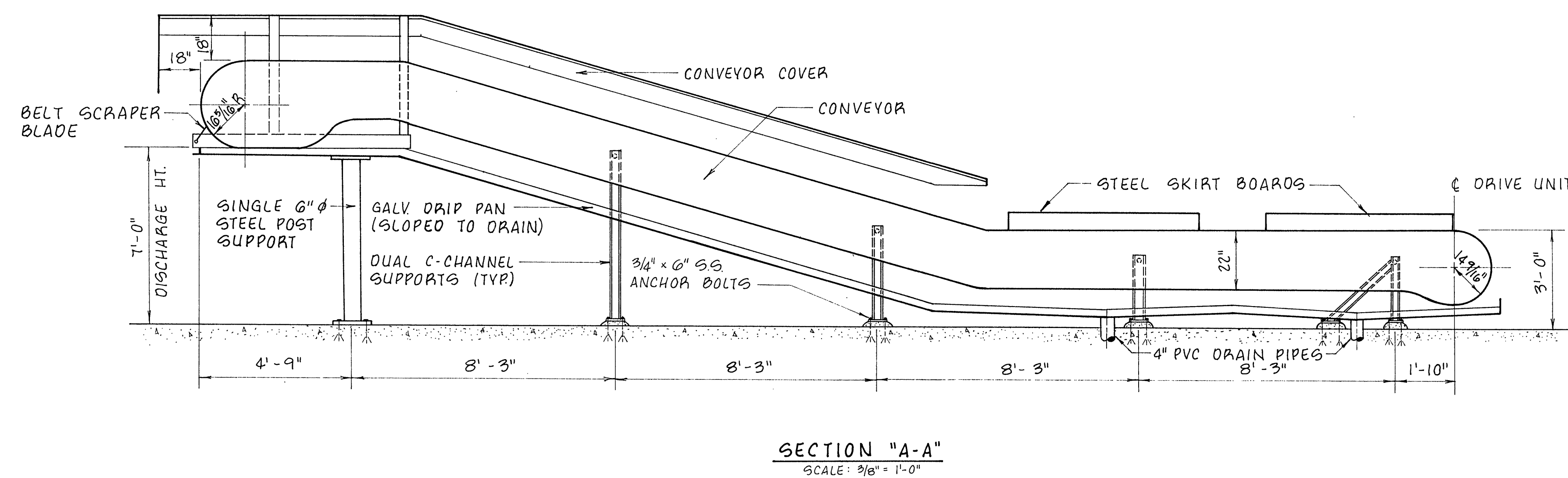
SERPENTINE BELT CONVEYOR
