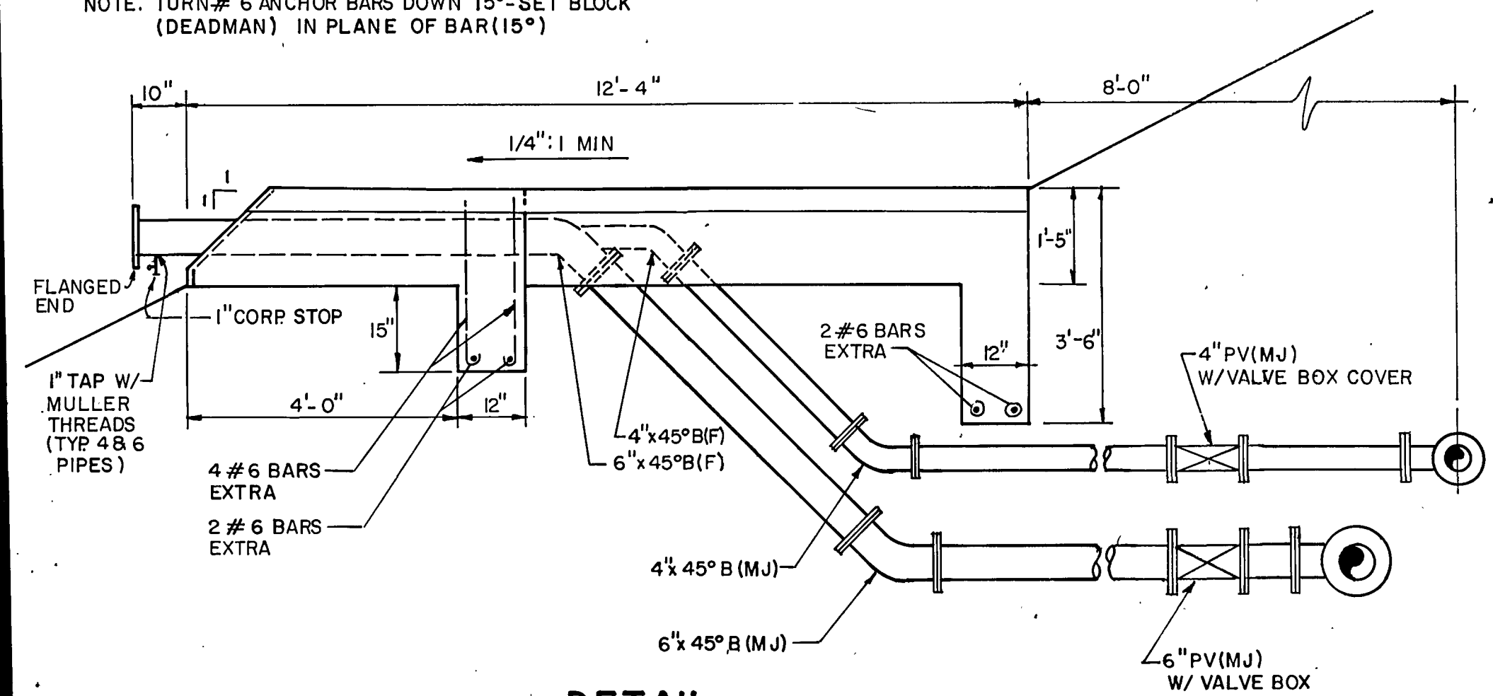
DETAIL FLEXIBLE PIPE CONNECTION AT BARGE CONTROL STATION N.T.S.
