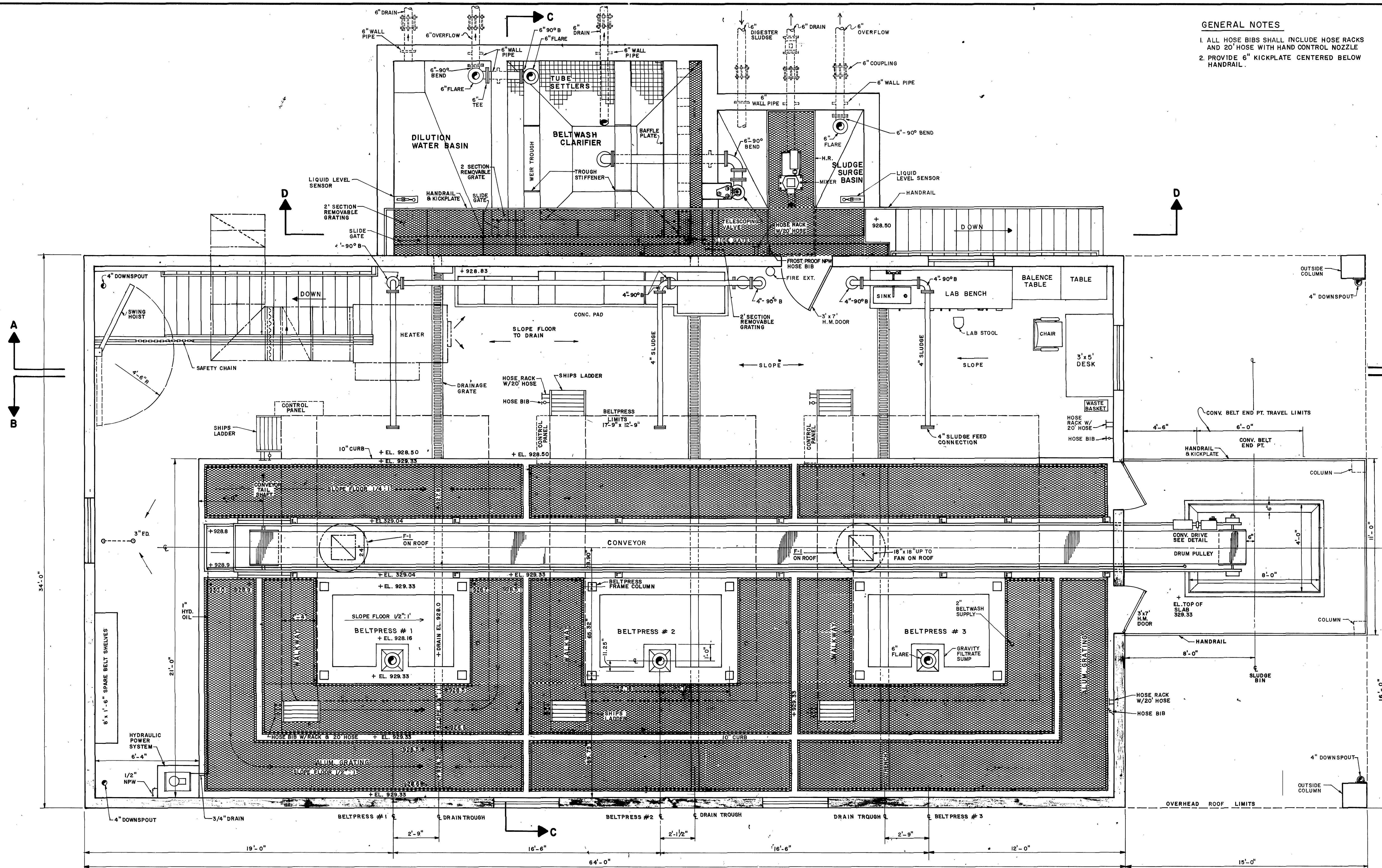
UPPER LEVEL FLOOR PLAN
