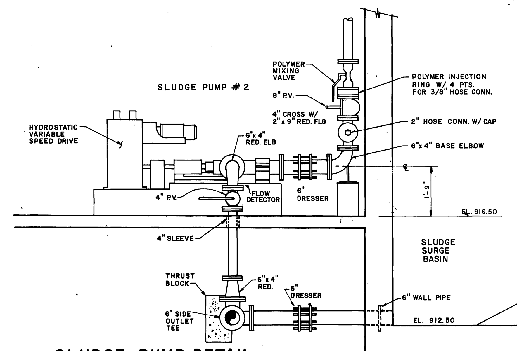
SLUDGE PUMP DETAIL SCALE: 1/2" = 1'-0"
