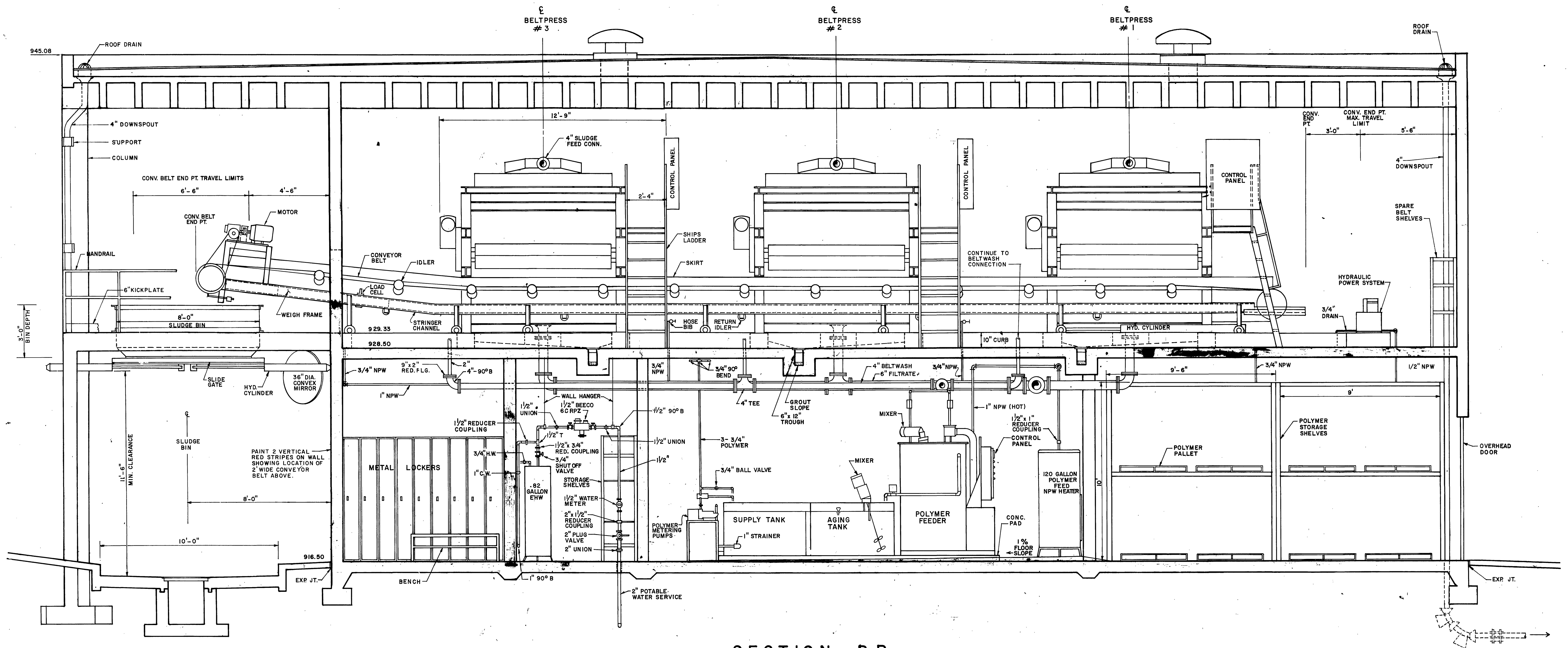
SECTION BB
