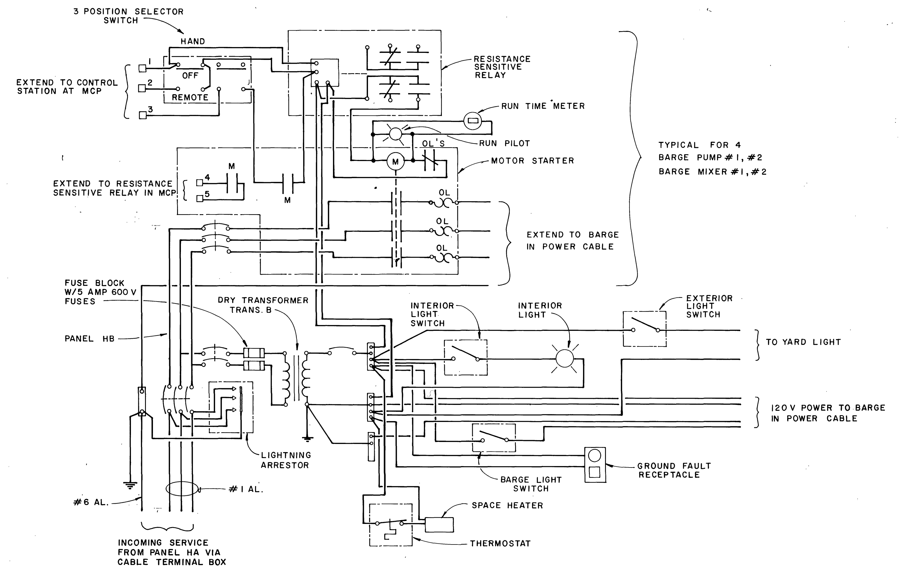
SCHEMATIC WIRING, BARGE CONTROL STATION
