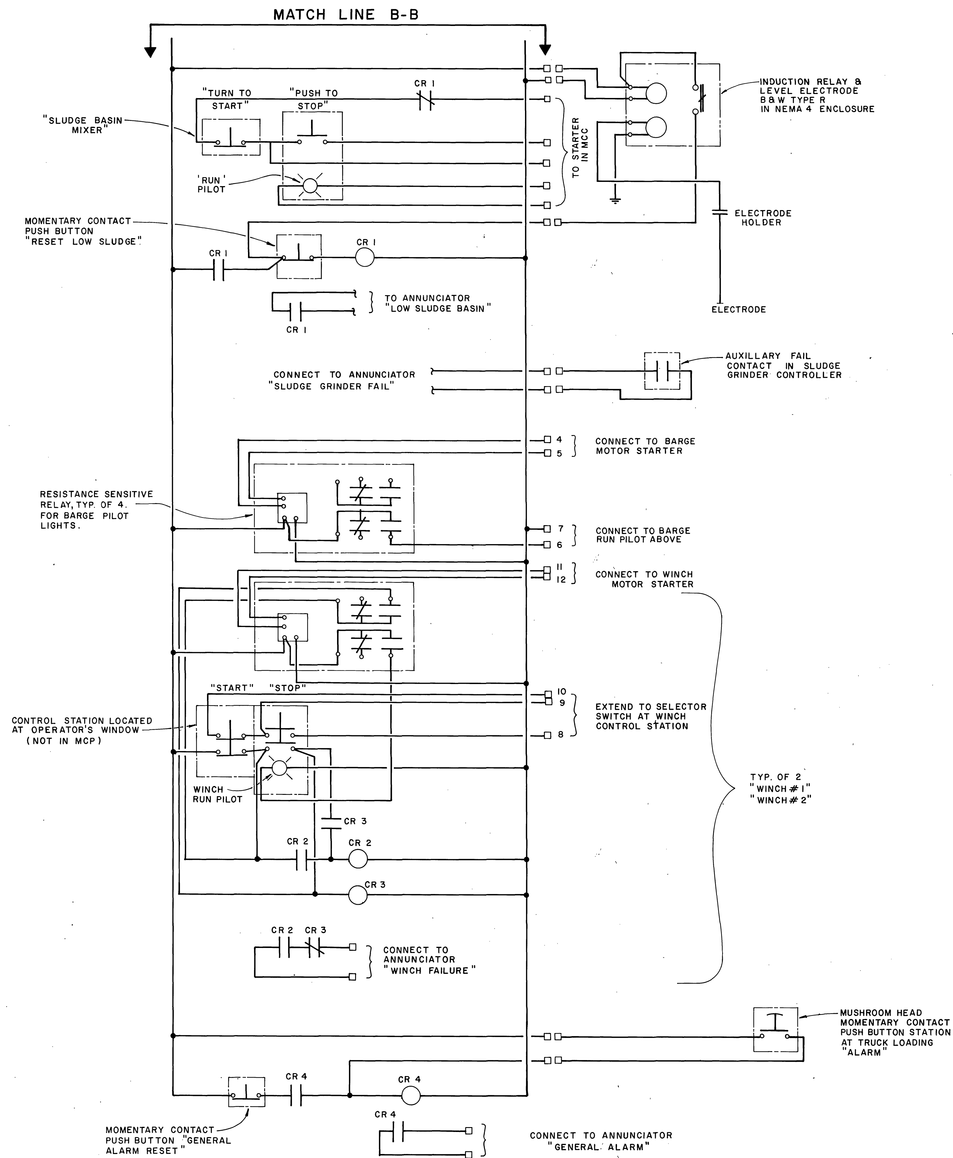
SCHEMATIC WIRING, MAIN CONTROL PANEL 'MCP' AND ASSOCIATED COMPONENTS
