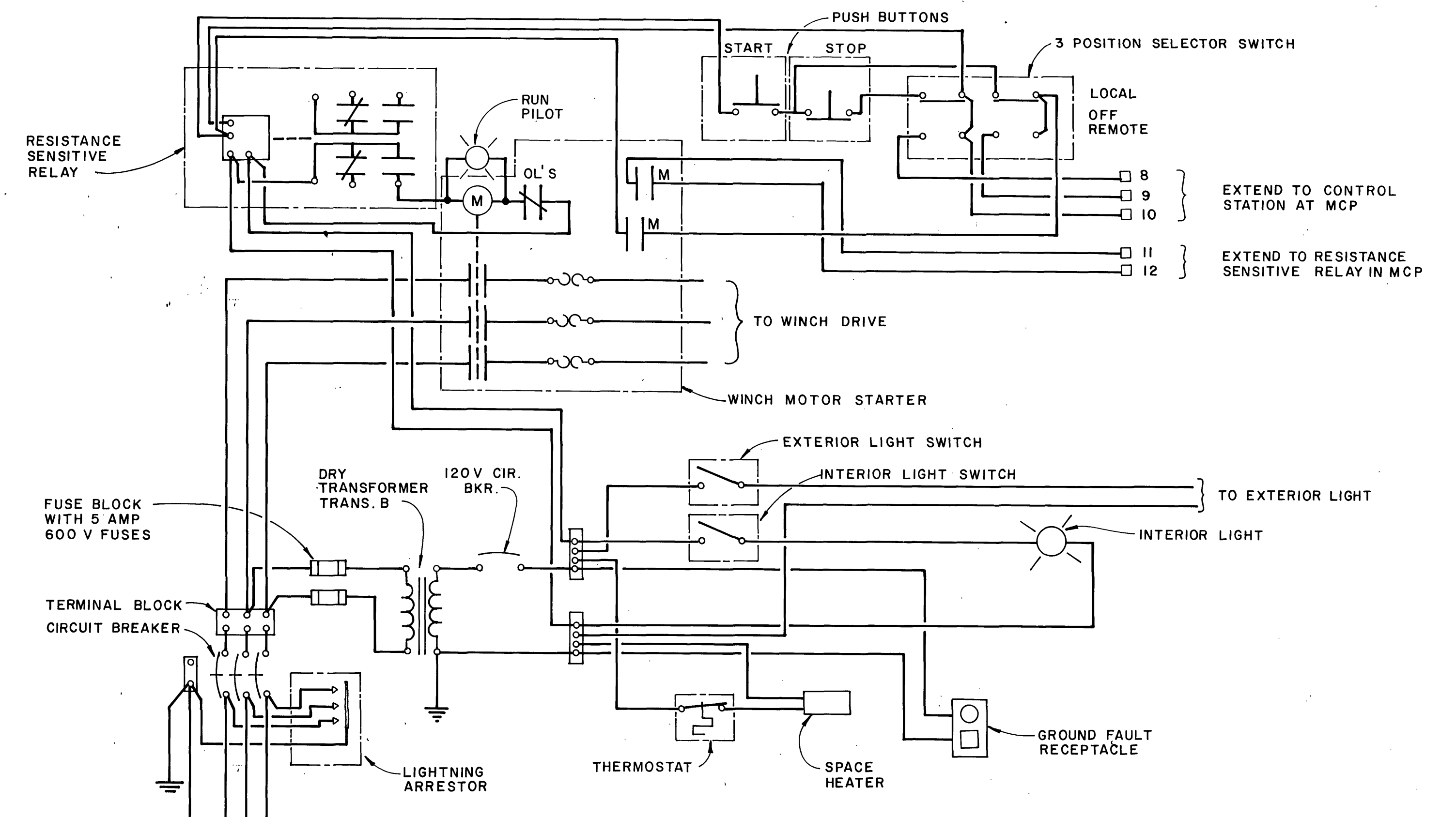
SCHEMATIC WIRING, WINCH CONTROL STATION
