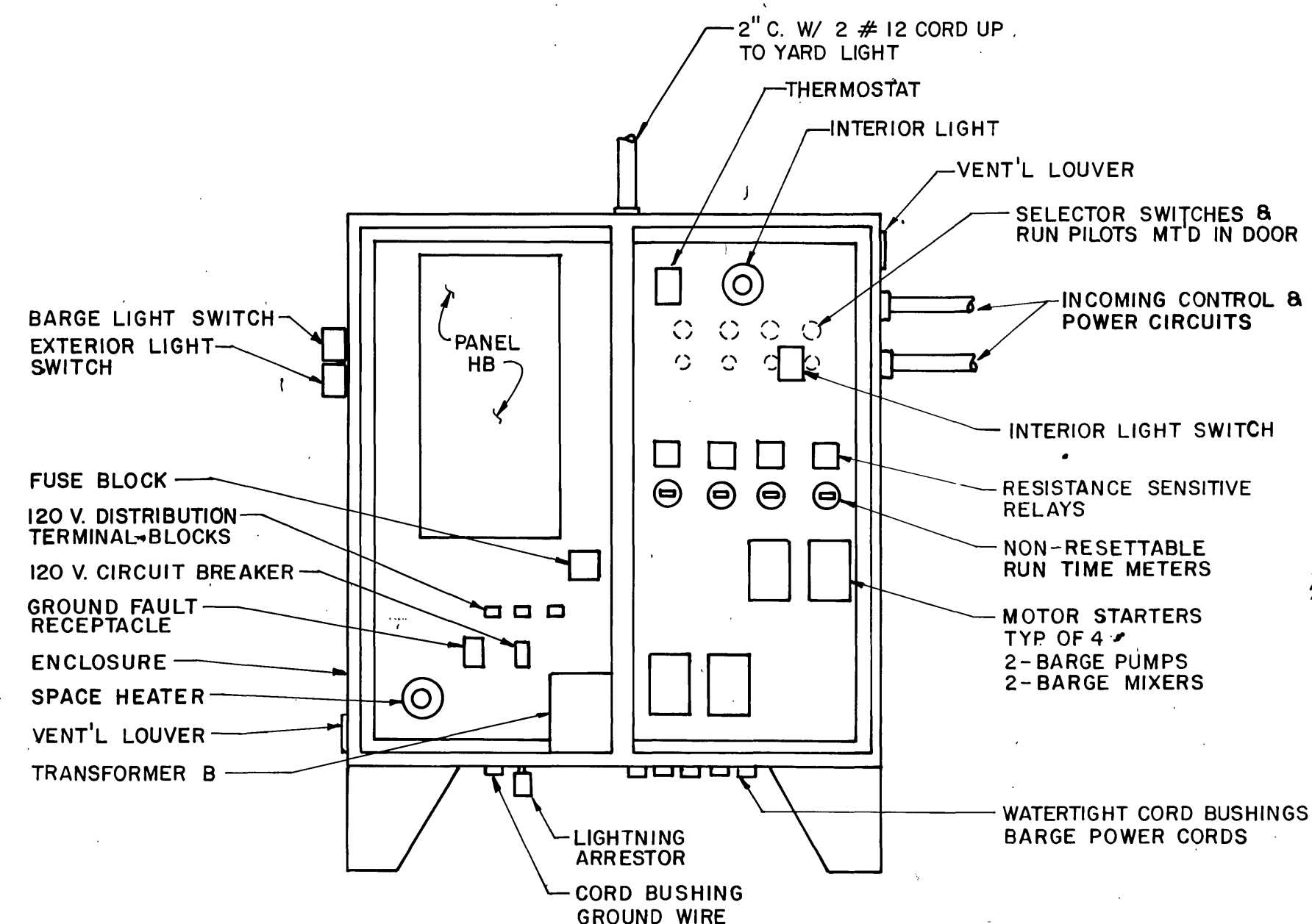
ELEVATION BARGE CONTROL STATION SHOWING COMPONENTS SEE SCHEDULE FOR DESCRIPTION N.T.S.
