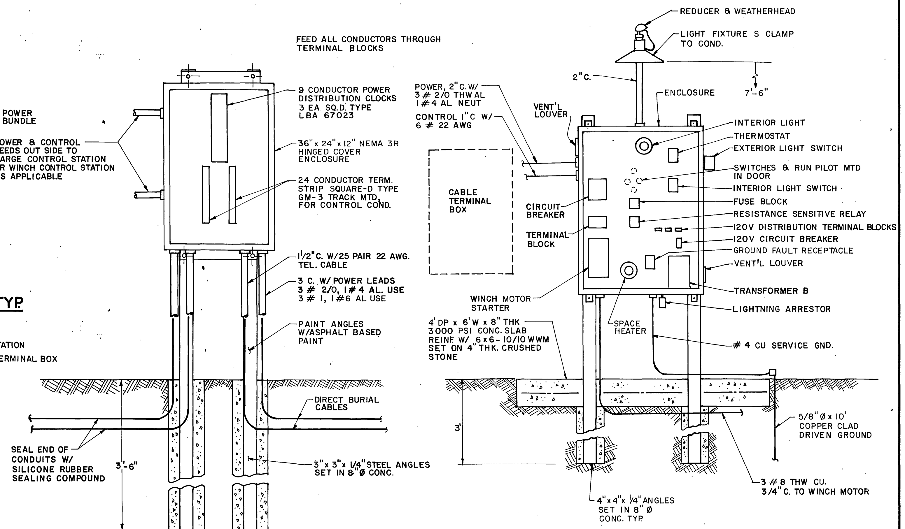
ELEVATION, WINCH CONTROL STATION SCALE: 3/4" = 1'-0"
