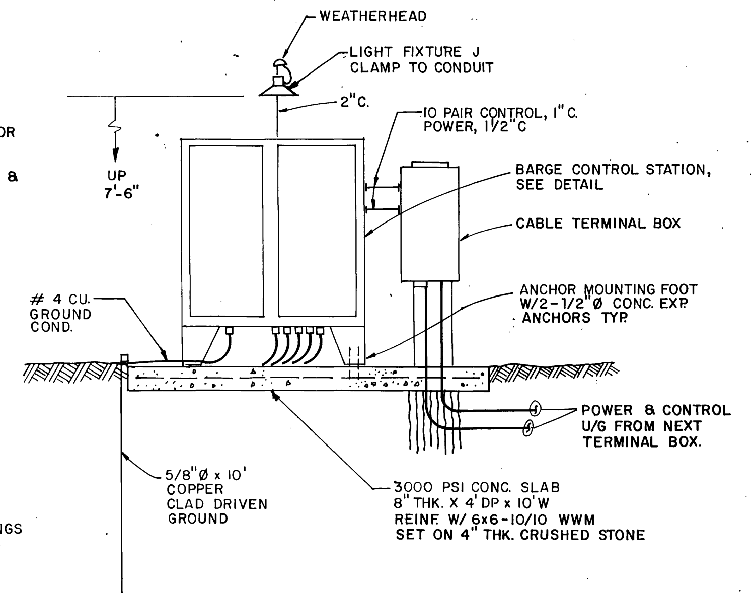
ELEVATION BARGE CONTROL STATION INSTALLATION N.T.S.
