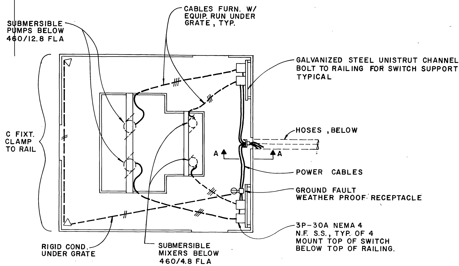
BARGE ELECTRICAL PLAN SCALE: 3/4" = 1'-0"
